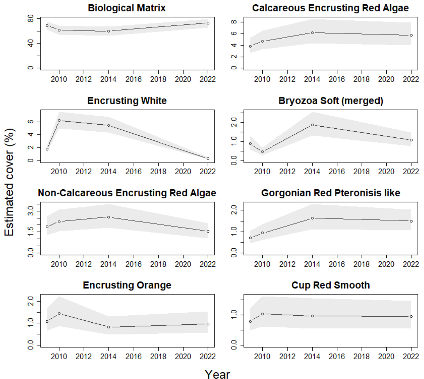
Figure 14. Model-based estimate of the temporal trend in the cover of the eight dominant morphospecies (including the grouping of biological matrix and soft bryozoa) in the Huon_13 site. Points and lines show the mean and shaded area shows the 95% credible intervals. Estimates were made at the mean depth of the transect, ignoring any spatial effects. Note the differing scales on the y-axes.
