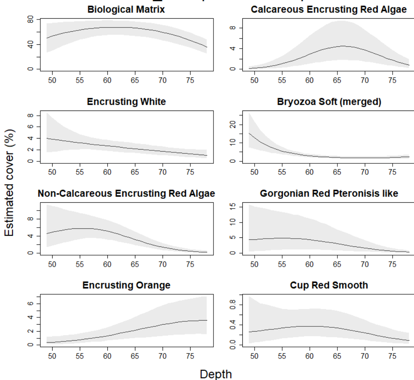
Figure 13. Relationship between the cover of the eight dominant morphospecies (including the grouping of biological matrix and soft bryozoa) with depth in the Huon_12 transect. Line shows the mean and shaded area shows the 95% credible intervals.
