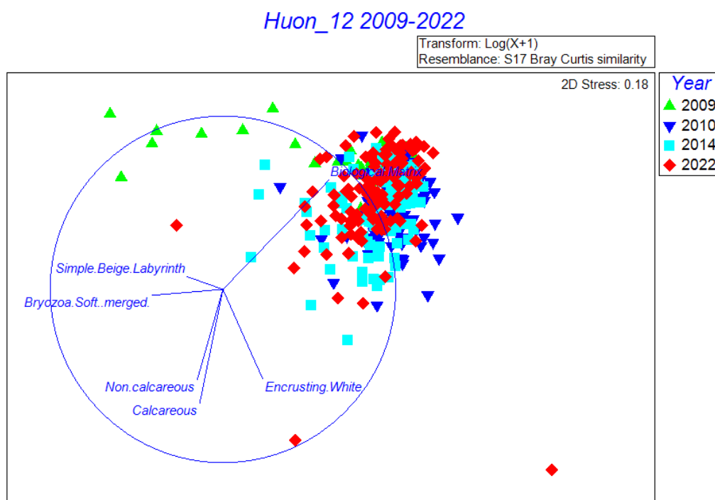
Figure 10. Non-metric multidimensional scaling plot showing community composition in Huon_12 transect across survey years.
