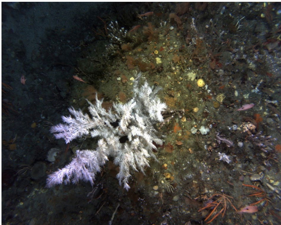
Figure 94. High profile reef with large black coral and branching sponges
