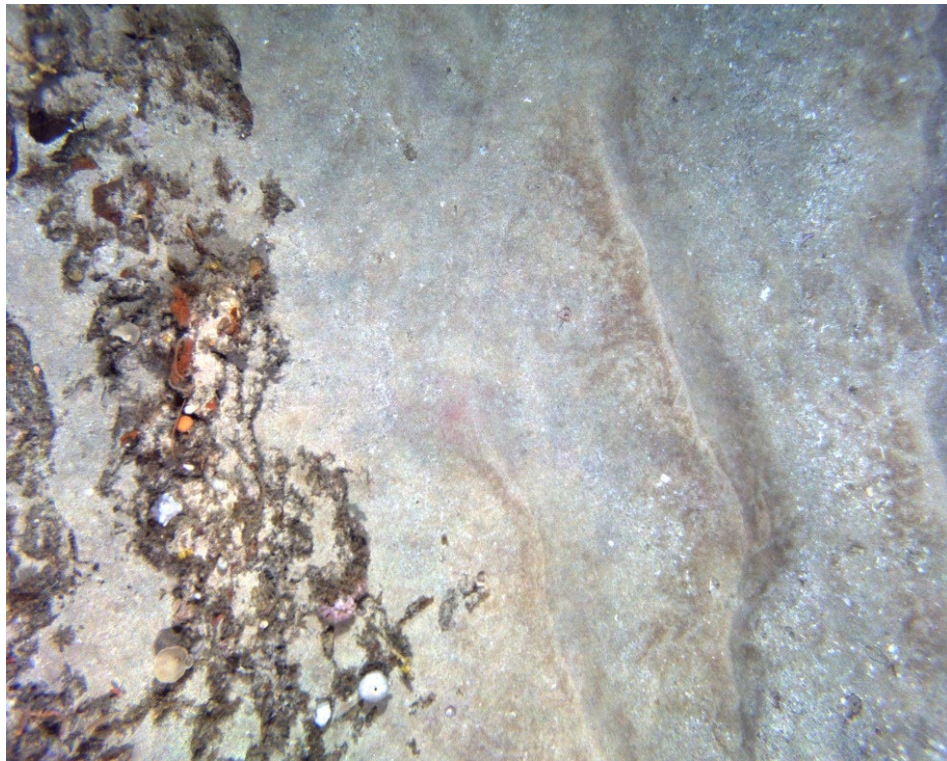
Figure 75. Low profile mixed habitat with rippled sand and sand inundated reef with sponge and biological matrix
