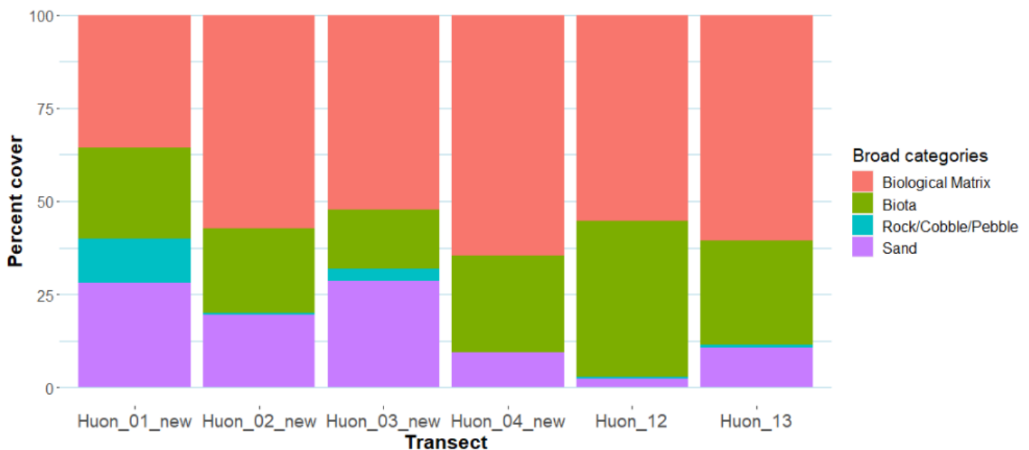
Figure 3. Broad categories of physical and biological characteristics present in each AUV transect in the Huon Marine Park
