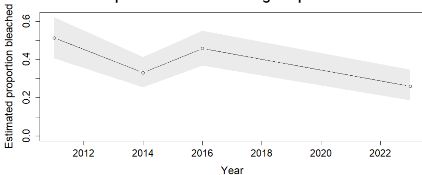
Figure 48. Temporal trend in the proportion of bleaching in cup red smooth sponges at Joe's Reef from targeted scoring.
