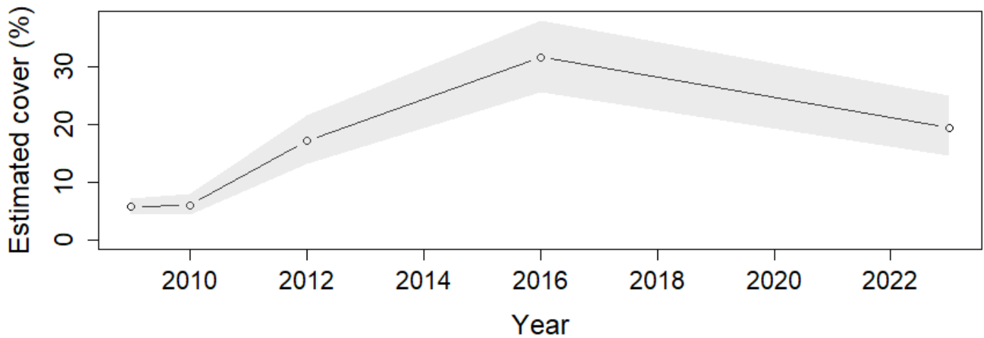
Figure 42. Model-based estimate of the temporal trend in the cover of Biological Matrix at AMP site 2. Points and lines show the mean and shaded area shows the 95% credible intervals. Estimates were made at the mean depth of the transect, ignoring any spatial effects.
