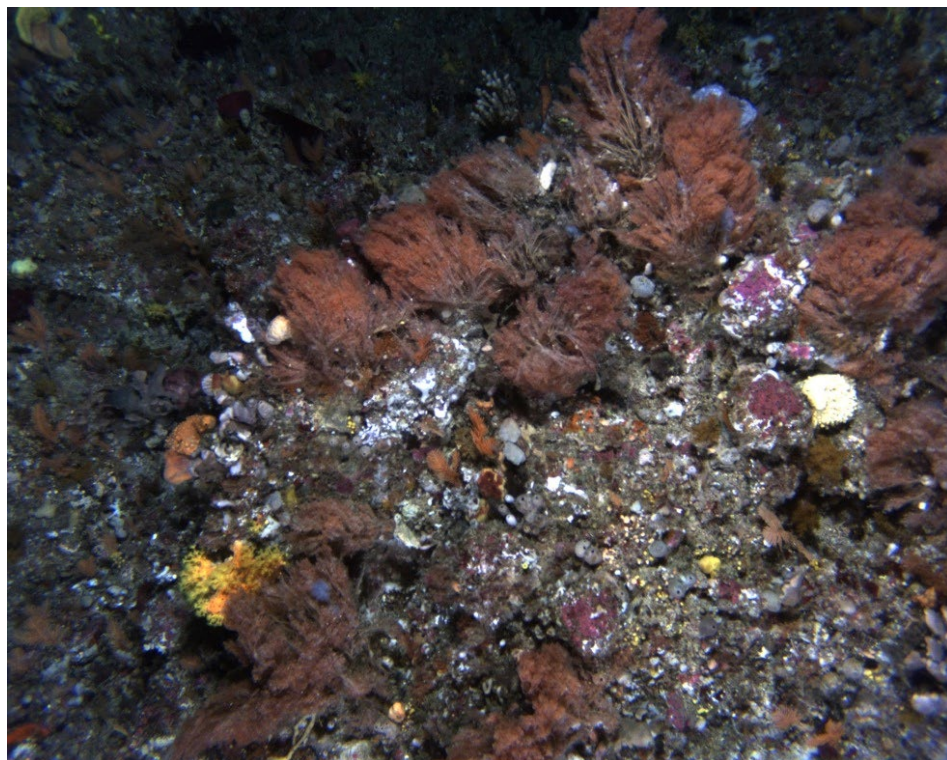
Figure 58. Branching orange sponge and soft bryozoan on flat sandy habitat
