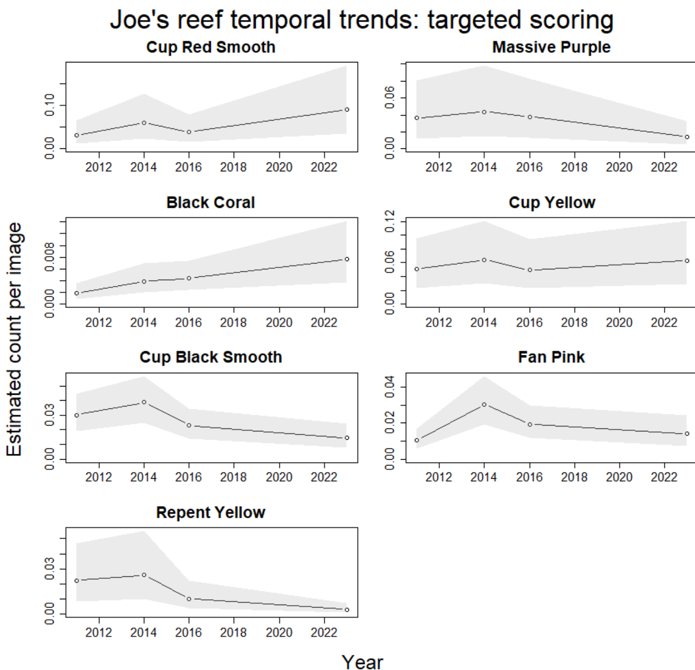
Figure 44. Model-based estimate of the temporal trend in the abundance of the seven morphospecies target scored at Joe's Reef. Points and lines show the mean and shaded area shows the 95% credible intervals. Estimates were made at the mean depth of the transect, ignoring any spatial effects. Note the different y-axes scales.
