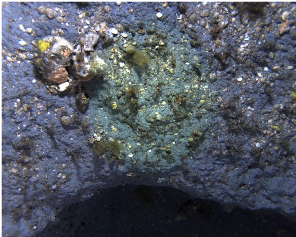
Figure 97. Bivalve shell dominated substrate with sponge
