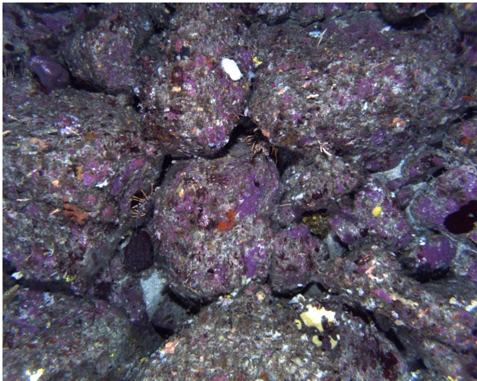
Figure 67. Southern rock lobsters amongst encrusting algae covered boulders
