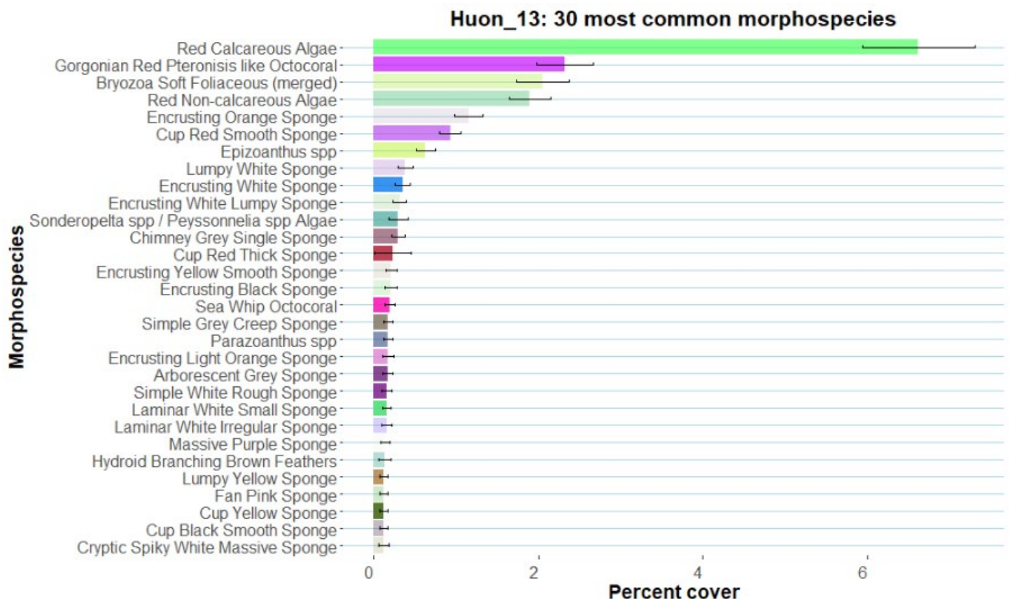
Figure 9. Percent cover (and standard error) of the 30 most common morphospecies annotated in the Huon_13 transect in Huon Marine Park AUV imagery. The biological matrix category was excluded from the plot for improved visualisation.
