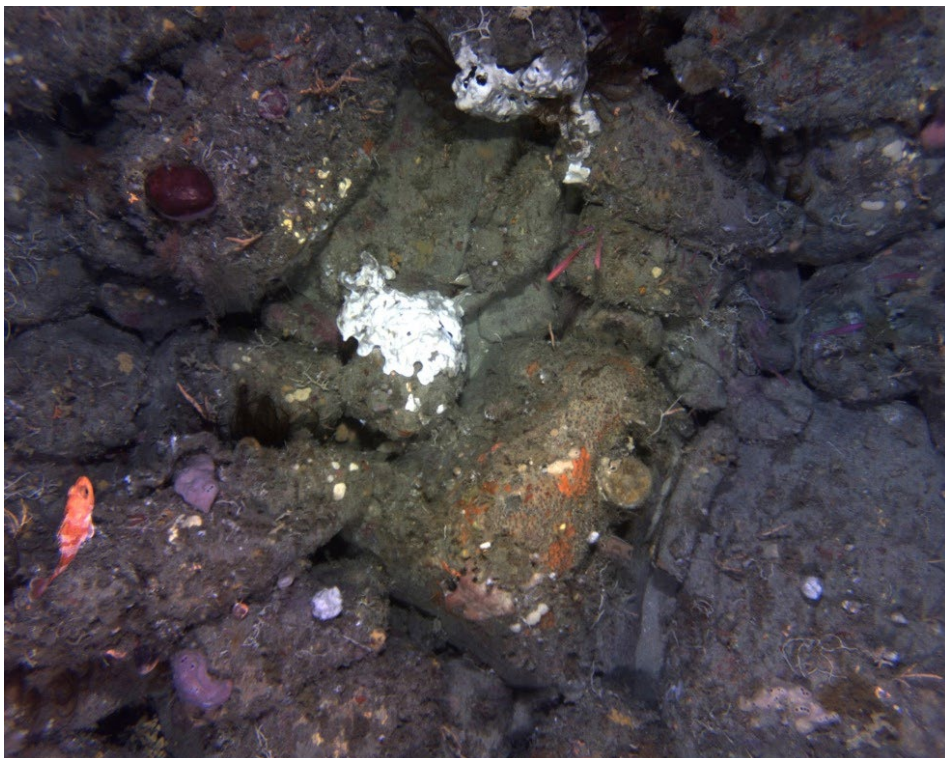
Figure 92. Boulder reef habitat with encrusting white and orange sponges and cup sponges
