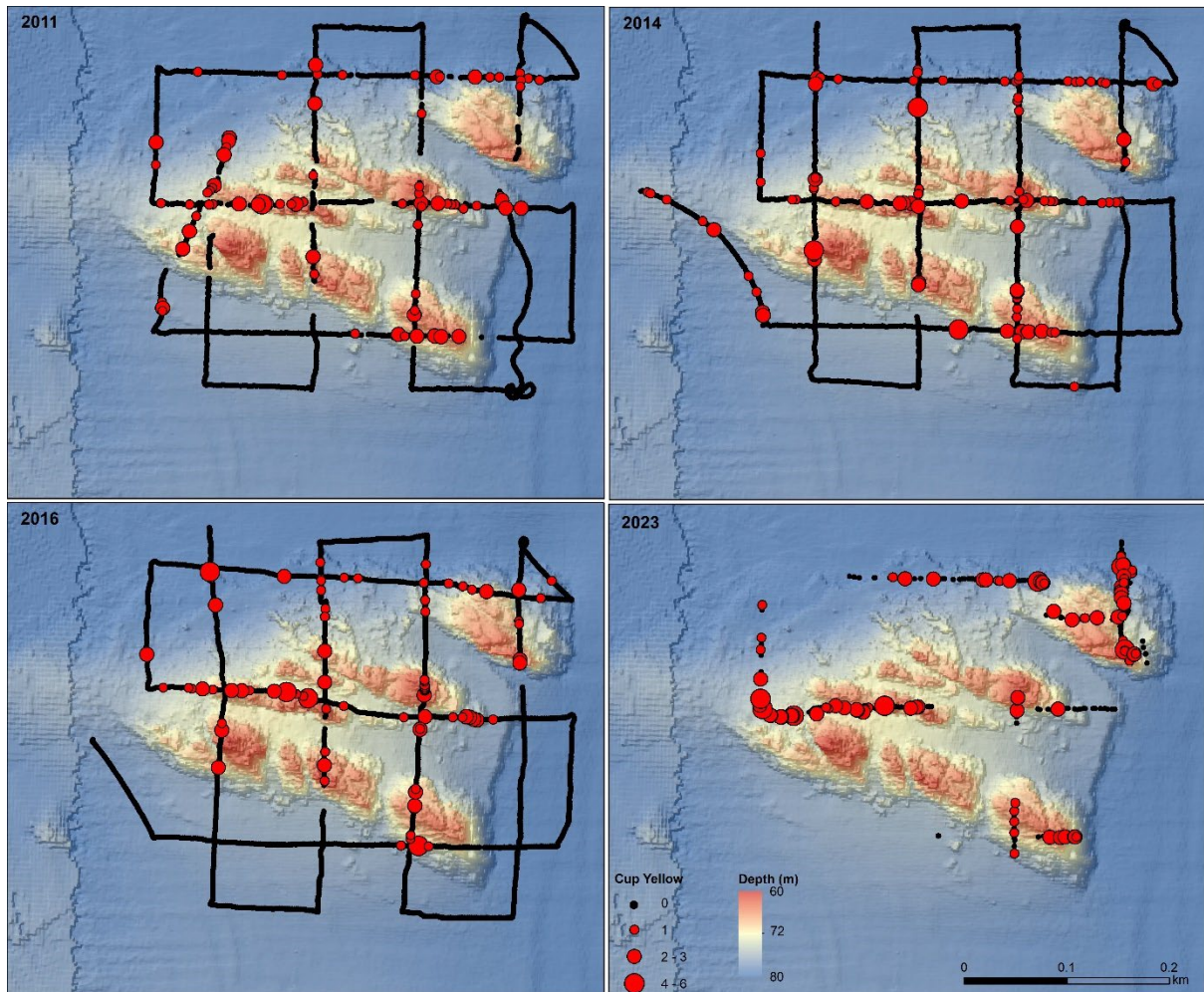
Figure 53. Changes in the spatial distribution in abundance (count per image) of cup yellow sponges at Joe's Reef from targeted scoring. Note that the 2023 survey had incomplete coverage due to regular AUV failure in this complex terrain.
