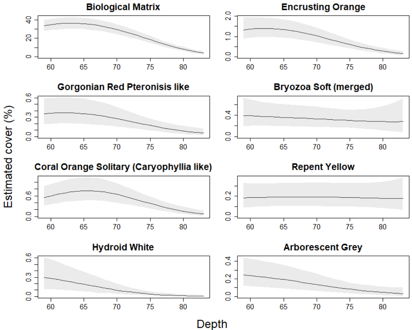
Figure 39. Relationship between the cover of the eight dominant morphospecies (including the grouping of biological matrix and soft bryozoa) with depth at Joe's Reef. Line shows the mean and shaded area shows the 95% credible intervals. Note the differing scales on the y-axes.
