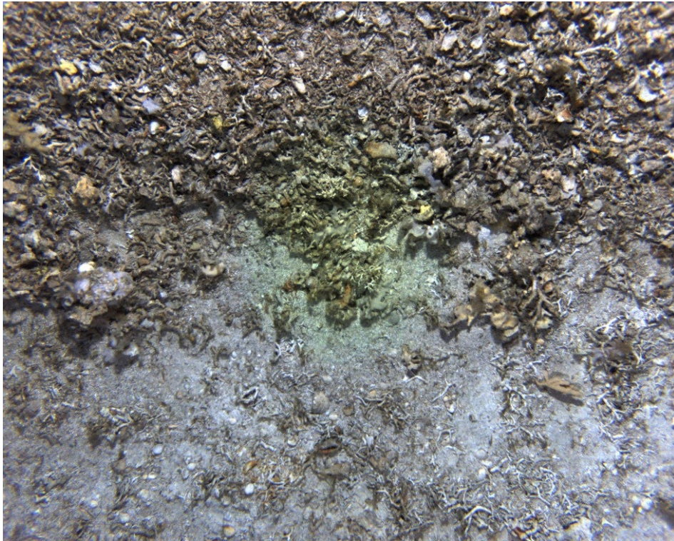
Figure 95. Bryozoan rubble and sand habitat with sponges
