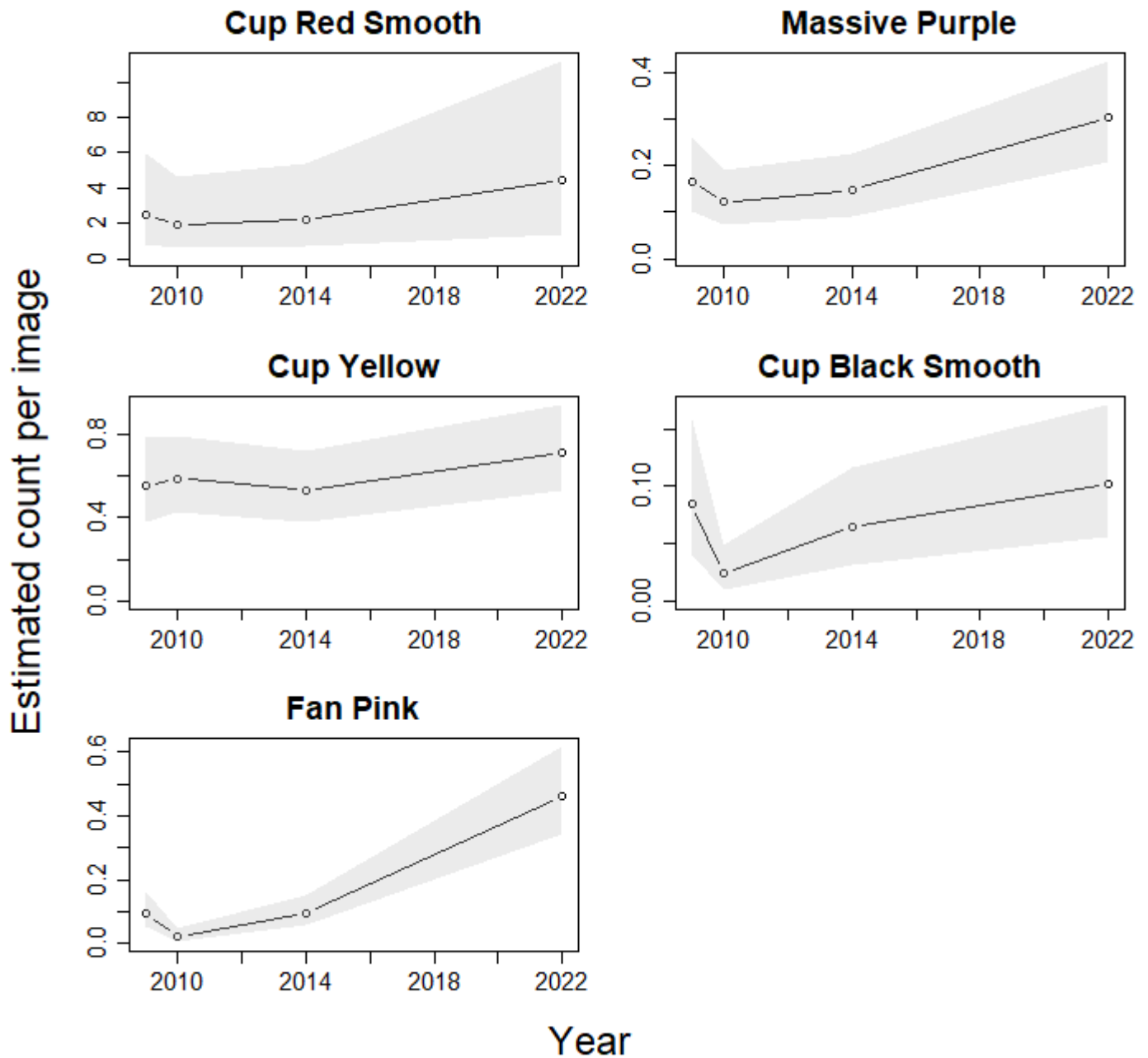
Figure 16. Model-based estimate of the temporal trend in the abundance of the five morphospecies target scored at the Huon_13 site. Points and lines show the mean and shaded area shows the 95% credible intervals. Estimates were made at the mean depth of the transect, ignoring any spatial effects.
