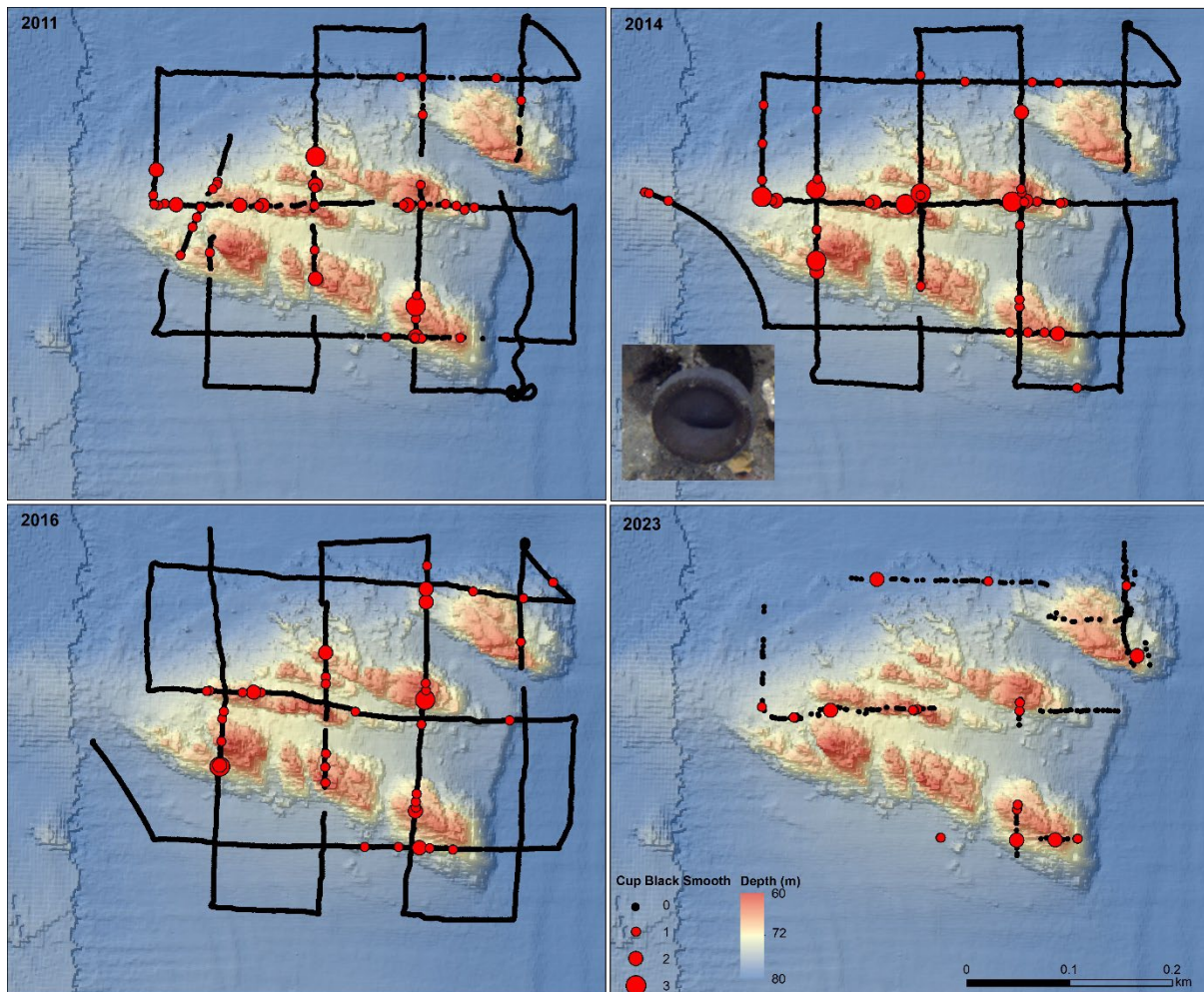
Figure 52. Changes in the spatial distribution in abundance (count per image) of cup black smooth sponges at Joe's Reef from targeted scoring. Note that the 2023 survey had incomplete coverage due to regular AUV failure in this complex terrain.
