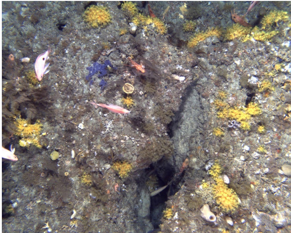
Figure 109. Rare outcropping low profile reef feature with Parazoanthids, sponges and soft bryozoa
