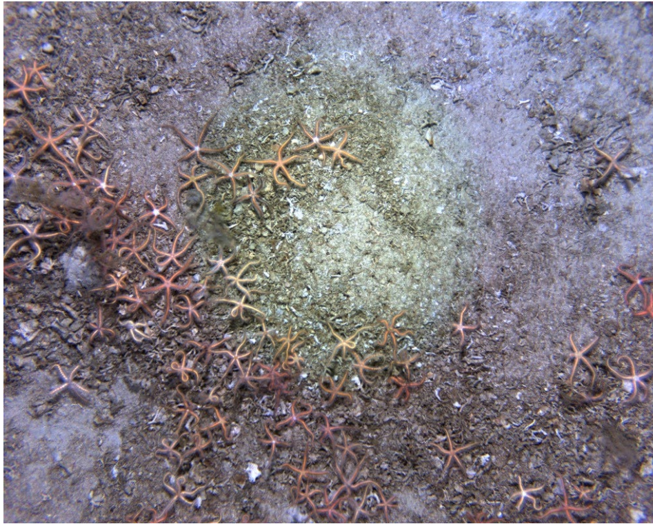
Figure 99. Sand and bryozoan rubble habitat with ophiuroids (brittle stars)
