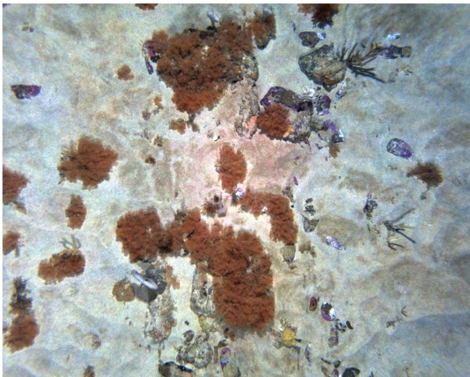
Figure 70. Low profile sand inundated reef with soft bryozoans and branching sponges
