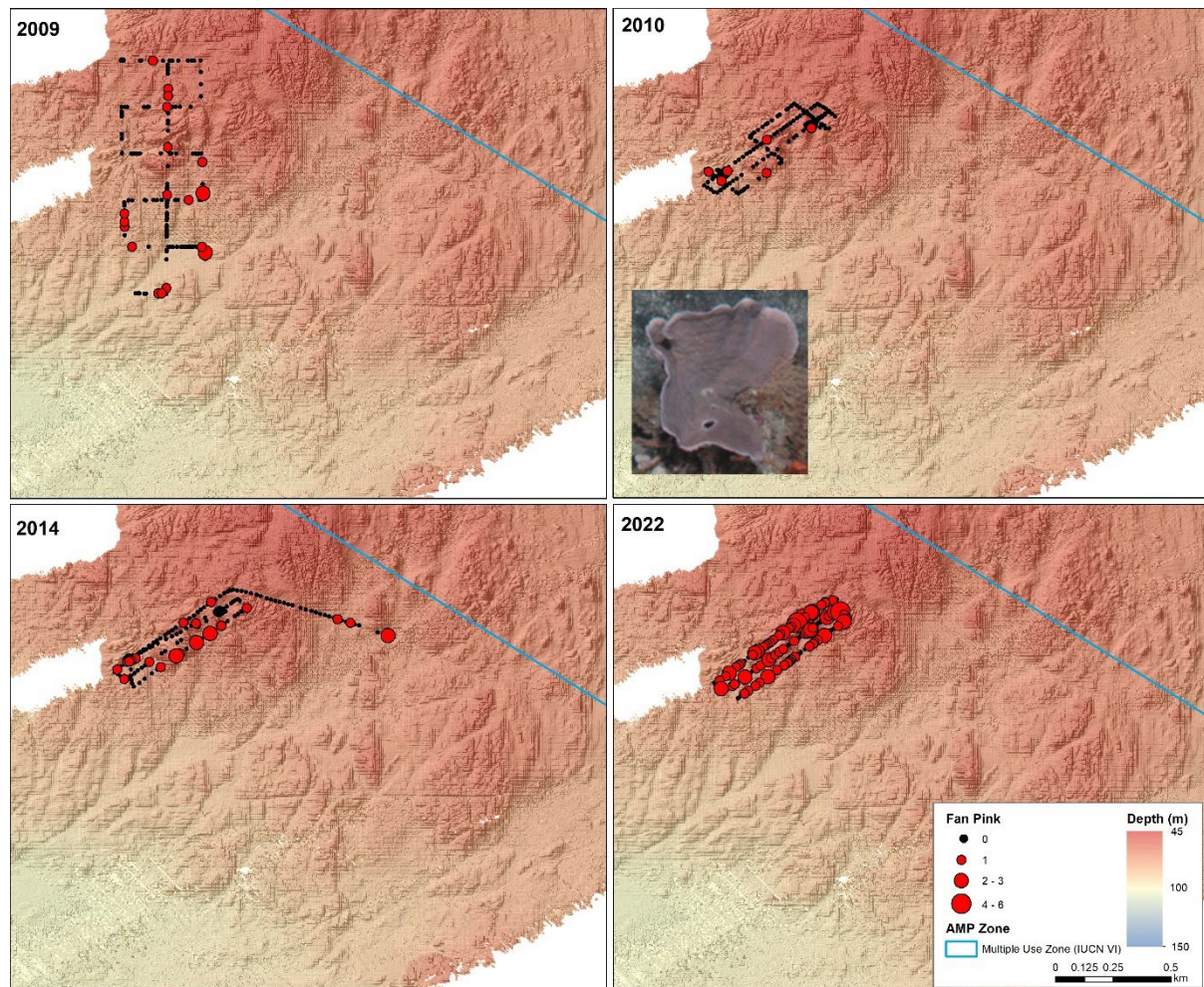
Figure 25. Changes in the spatial distribution in abundance (count per image) of fan pink sponges at Huon_13 transect from targeted scoring. Note that a different transect design was used in the 2009 survey compared to subsequent surveys.
