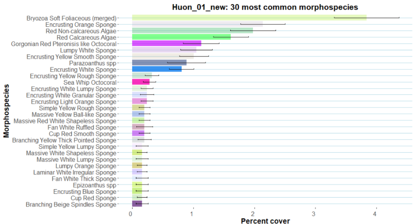
Figure 4. Percent cover (and standard error) of the 30 most common morphospecies annotated in the Huon_01_new transect in Huon Marine Park AUV imagery. The biological matrix category was excluded from the plot for improved visualisation.
