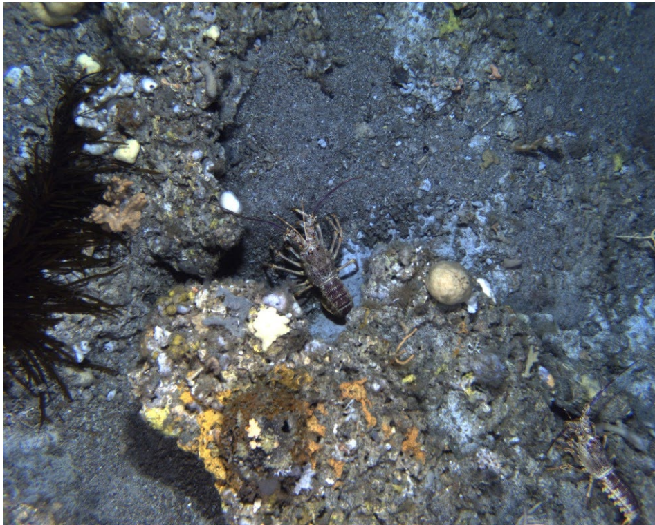
Figure 101. Low profile mudstone reef habitat with rock lobsters, encrusting sponges, and drift algae (phyllospora)
