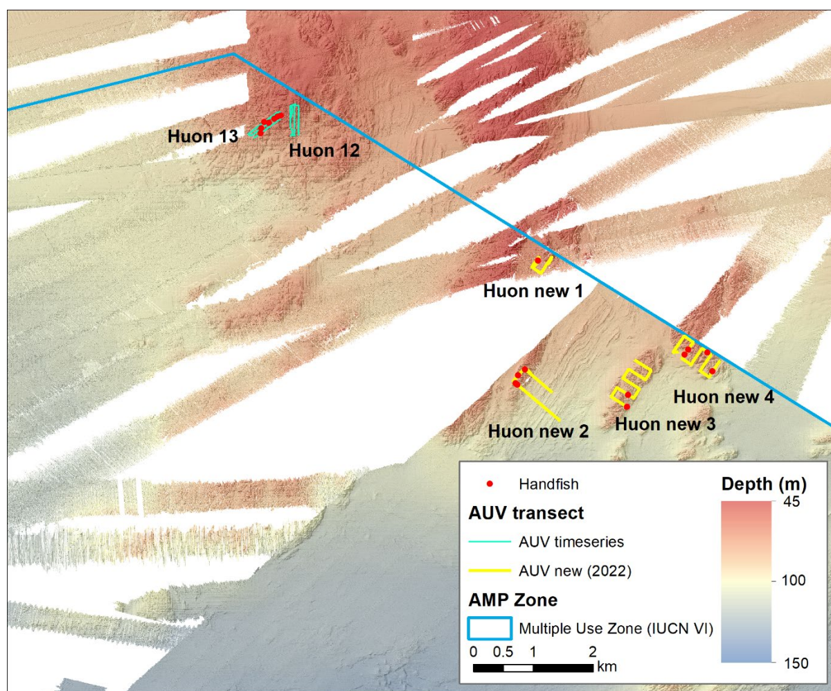
Figure 56. Location of handfish observed in Huon AMP
