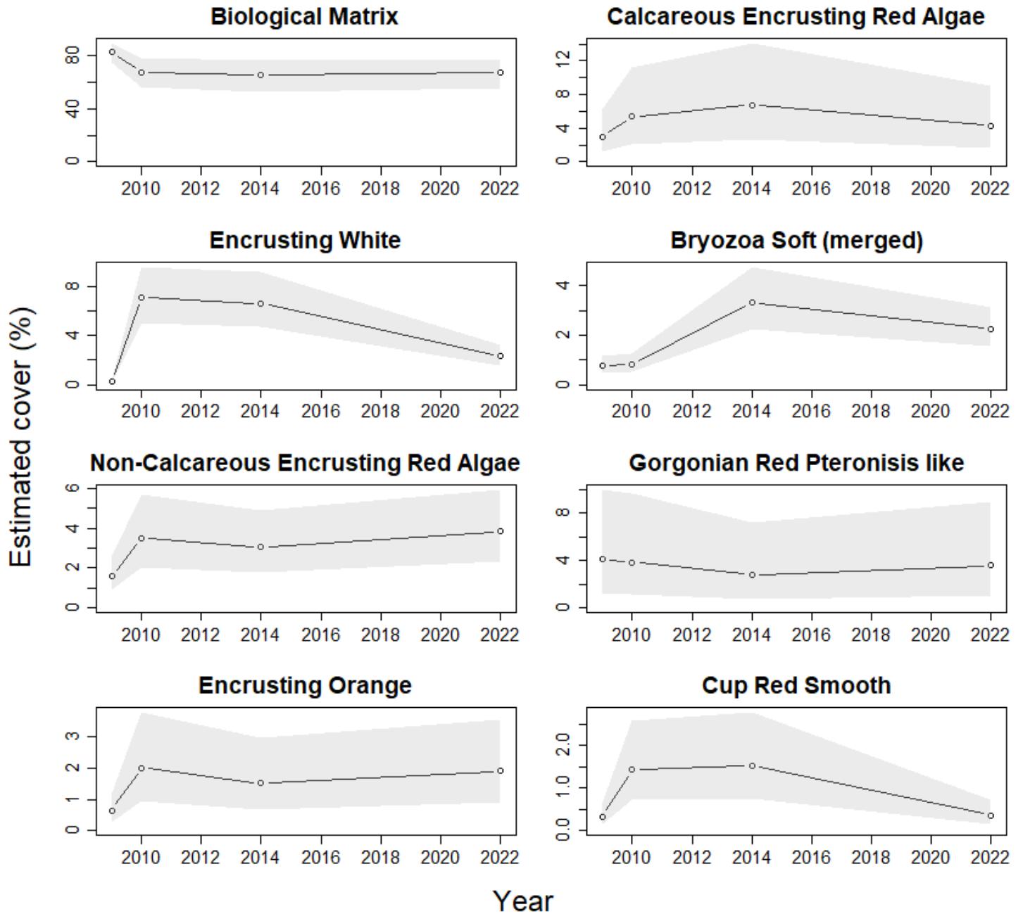
Figure 12. Model-based estimate of the temporal trend in the cover of the eight dominant morphospecies (including the grouping of biological matrix and soft bryozoa) in the Huon_12 transect. Points and lines show the mean and shaded area shows the 95% credible intervals. Estimates were made at the mean depth of the transect, ignoring any spatial effects.
