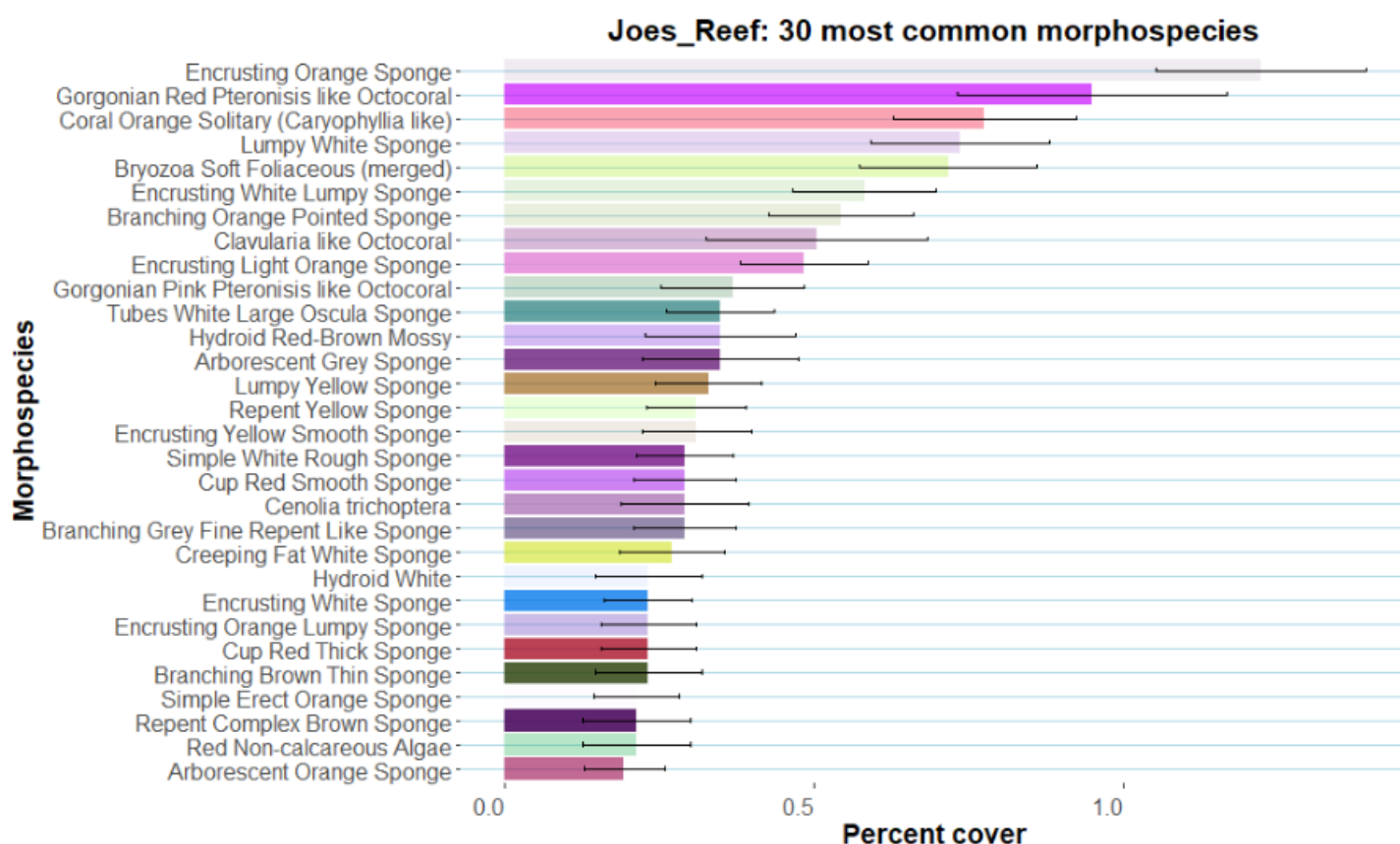
Figure 29. Percent cover (and standard error) of the 30 most common morphospecies at Joe's Reef. Biological matrix was excluded for improved visualisation.
