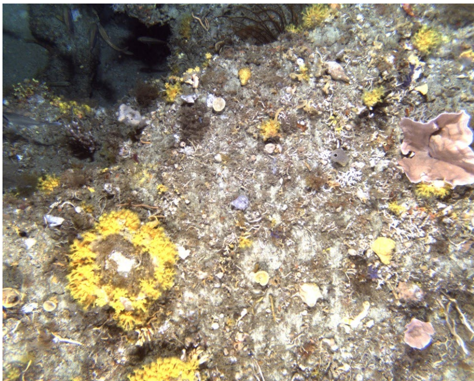
Figure 110. Rare outcropping low profile reef feature with Parazoanthids, fan pink sponges, soft bryozoa and biological matrix
