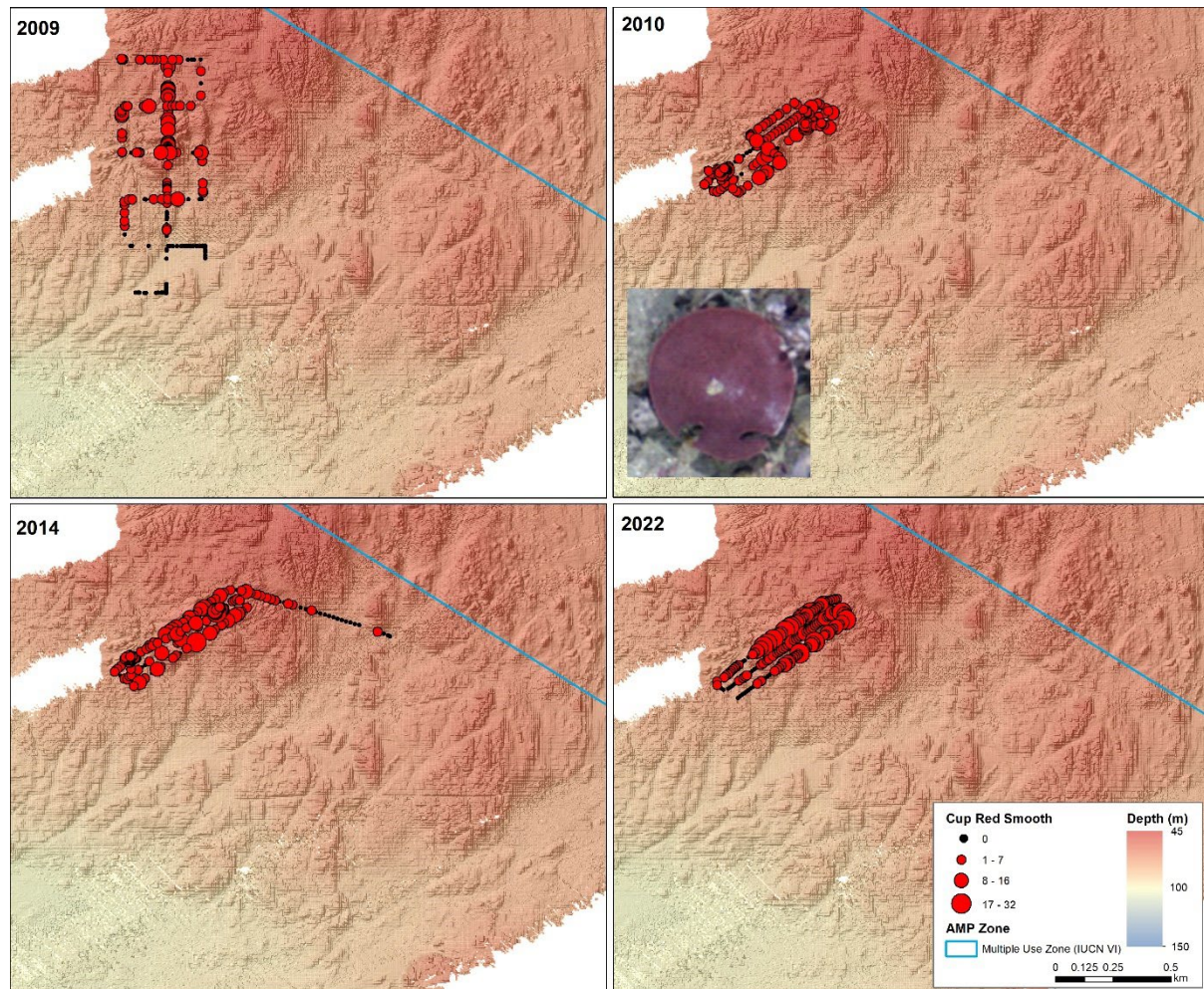
Figure 18. Changes in the spatial distribution in abundance (count per image) of cup red smooth sponges at Huon_13 transect from targeted scoring. Note that a different transect design was used in the 2009 survey compared to subsequent surveys.
