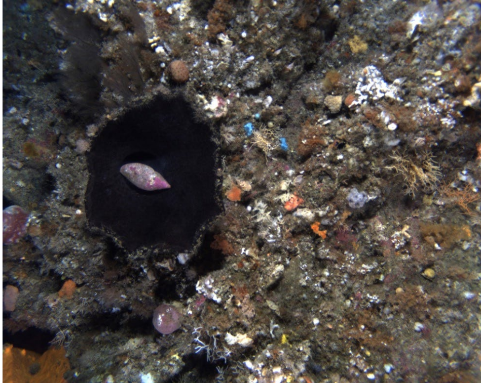
Figure 77. Reef with large black smooth cup sponge, soft bryozoa, bramble corals and biological matrix
