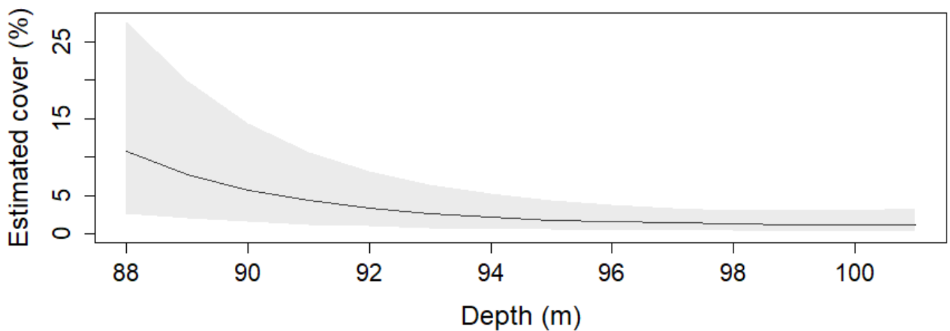
Figure 41. Relationship between the cover of biological matrix and depth at AMP site 1. Line shows the mean and shaded area shows the 95% credible intervals.
