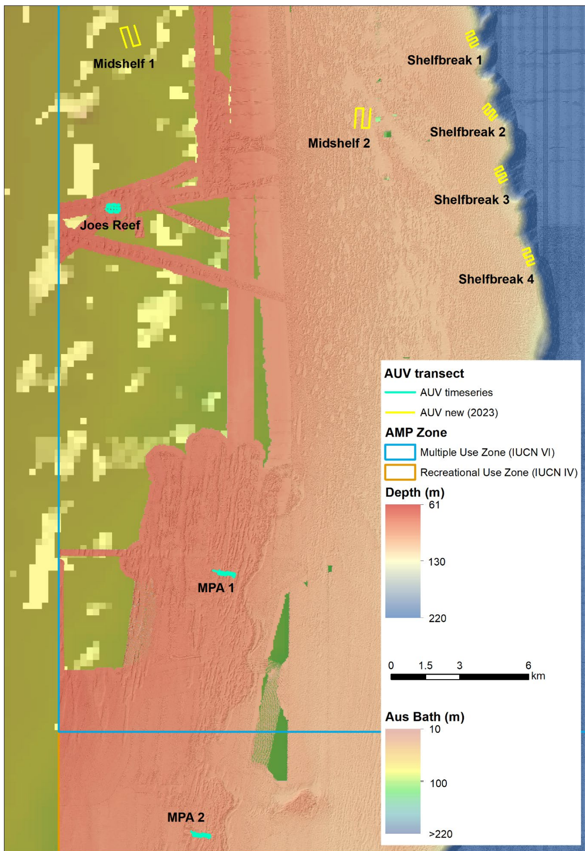
Figure 26. Locations of AUV transects in FMP, including repeat time series and new extended coverage.
