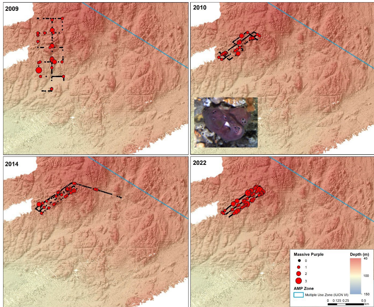
Figure 22. Changes in the spatial distribution in abundance (count per image) of massive purple sponges at Huon_13 transect from targeted scoring. Note that a different transect design was used in the 2009 survey compared to subsequent surveys.
