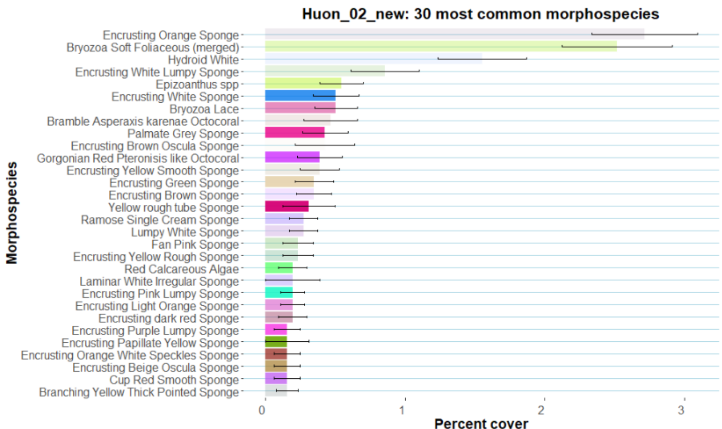
Figure 5. Percent cover (and standard error) of the 30 most common morphospecies annotated in the Huon_02_new transect in Huon Marine Park AUV imagery. The biological matrix category was excluded from the plot for improved visualisation.
