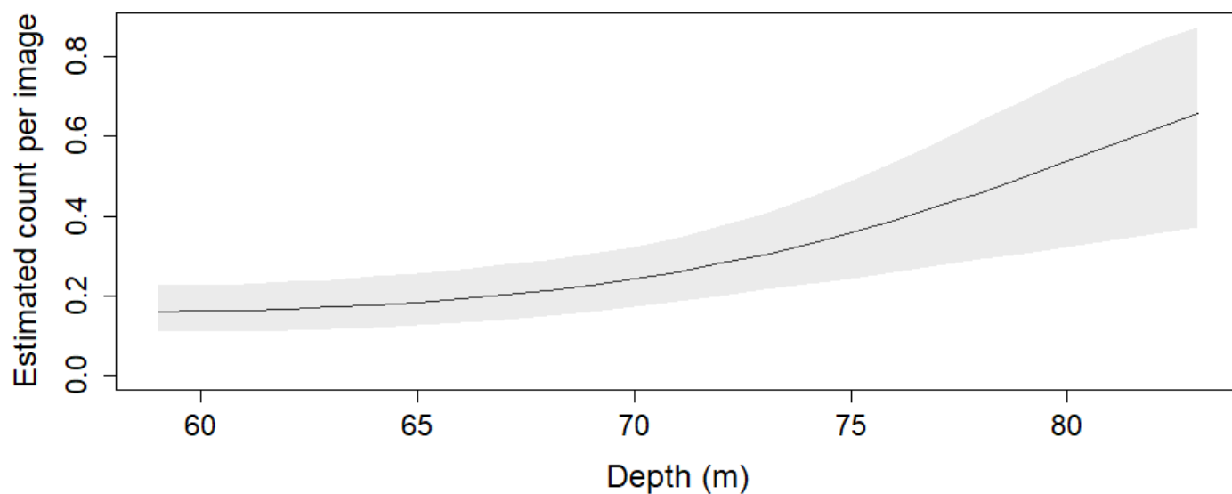
Figure 49. Depth relationship of bleaching from targeted scoring of cup red smooth sponges at Joe's Reef.
