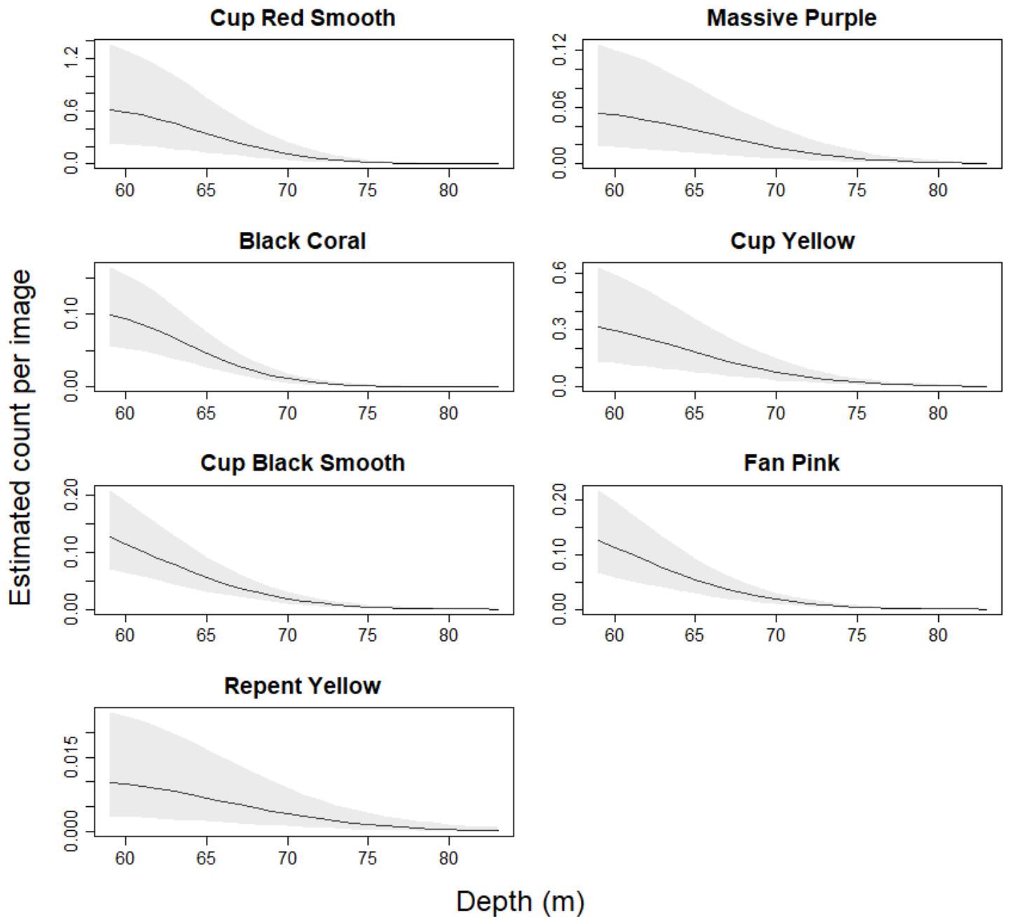
Figure 45. Relationship between the abundance of the seven target scored morphospecies with depth at Joe's Reef. Line shows the mean and shaded area shows the 95% credible intervals. Note the different y-axes scales.
