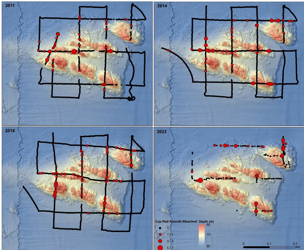
Figure 47. Changes in the spatial distribution in abundance (count per image) of bleached cup red smooth sponges at Joe's Reef from targeted scoring. Note that the 2023 survey had incomplete coverage due to regular AUV failure in this complex terrain.
