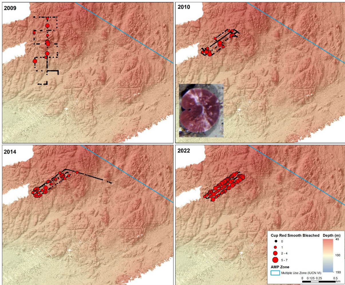
Figure 19. Changes in the spatial distribution in abundance (count per image) of bleached cup red smooth sponges at Huon_13 transect from targeted scoring. Note that a different transect design was used in the 2009 survey compared to subsequent surveys.
