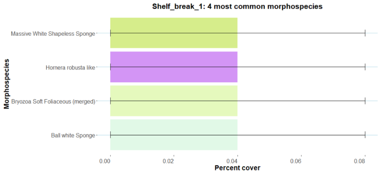
Figure 30. Percent cover (and standard error) of the four most common morphospecies at the Shelf break 1 transect. Biological matrix was excluded for improved visualisation.
