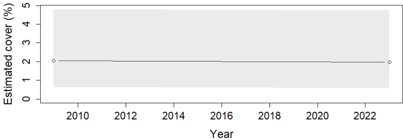
Figure 40. Model-based estimate of the temporal trend in the cover of Biological Matrix at AMP site 1. Points and lines show the mean and shaded area shows the 95% credible intervals. Estimates were made at the mean depth of the transect, ignoring any spatial effects.
