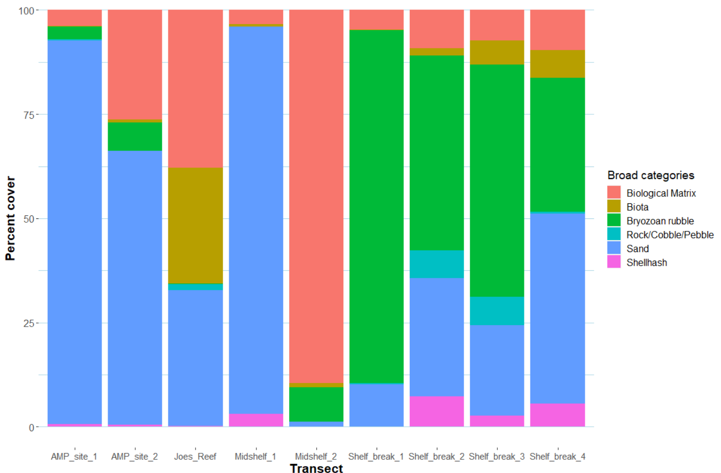
Figure 28. Summary of broad categories of physical substrate and biota scored across each transect in Freycinet Marine Park.
