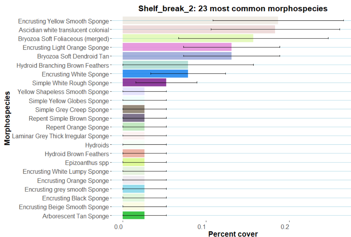
Figure 31. Percent cover (and standard error) of the twenty-three most common morphospecies at the Shelf break 2 transect. Biological matrix was excluded for improved visualisation.
