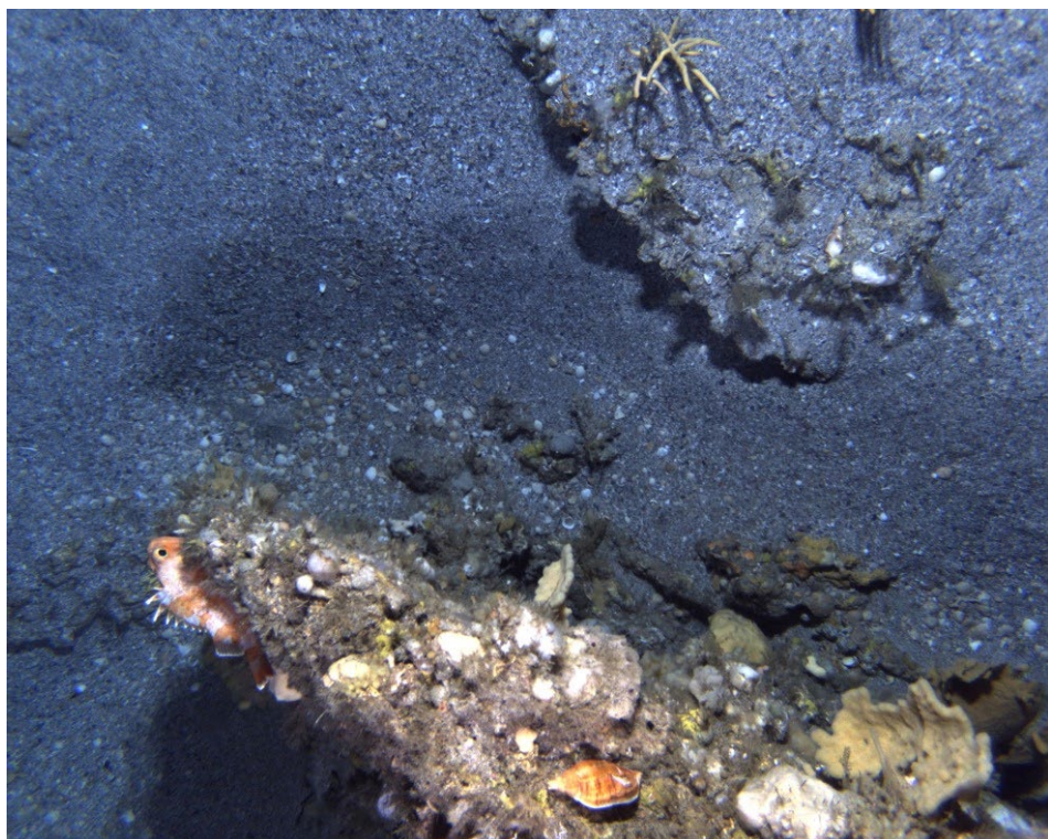
Figure 108. Moderate relief mixed habitat with laminar and branching sponges and ocean perch
