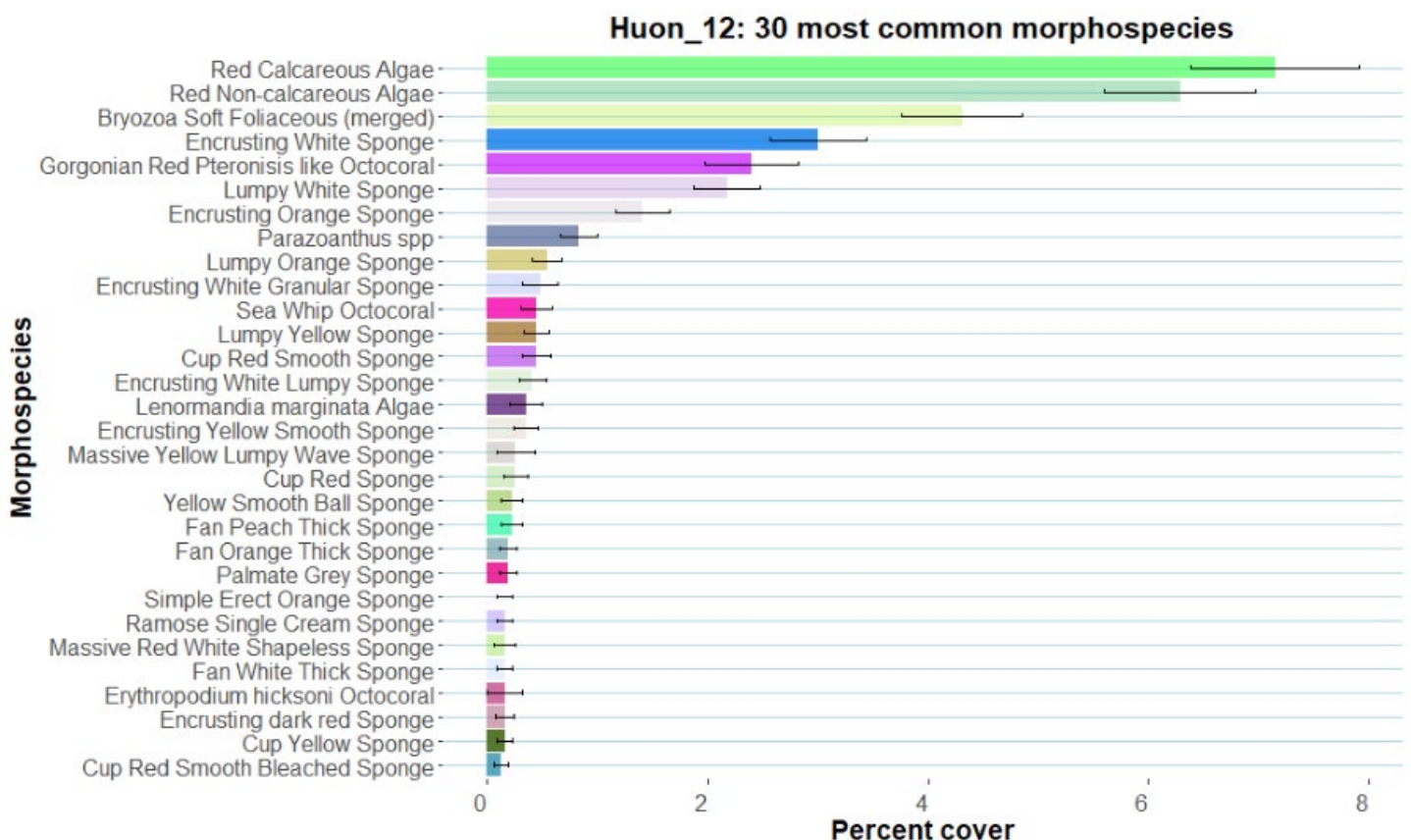
Figure 8. Percent cover (and standard error) of the 30 most common morphospecies annotated in the Huon_12 transect in Huon Marine Park AUV imagery. The biological matrix category was excluded from the plot for improved visualisation.
