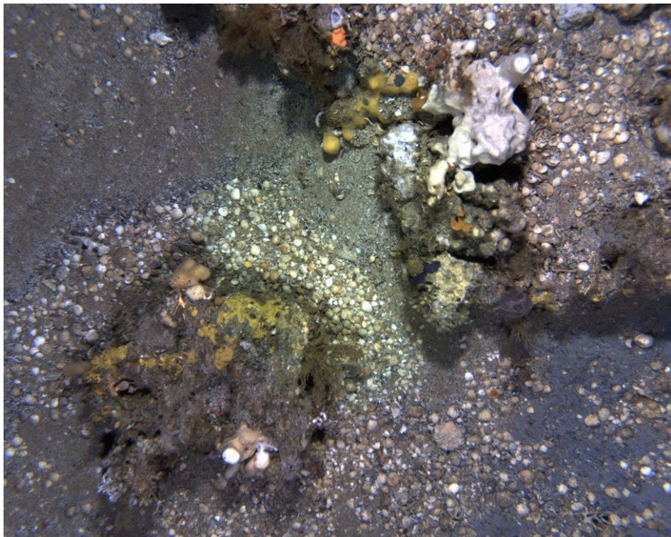
Figure 100. Mixed mudstone reef/sand/bivalve shell habitat with massive white lumpy sponge, encrusting yellow smooth sponge, and soft bryozoa including dendroid tan in the top of the image
