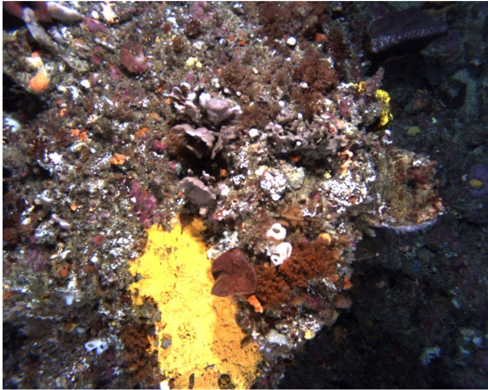
Figure 66. Matrix heavy high profile reef top with encrusting yellow smooth sponge, palmate grey and soft bryozoan
