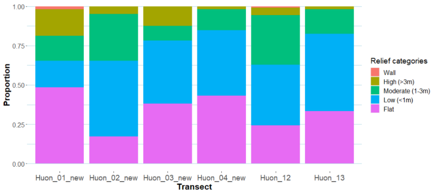
Figure 2. Proportions of different relief categories present across each transect in Huon Marine Park.
