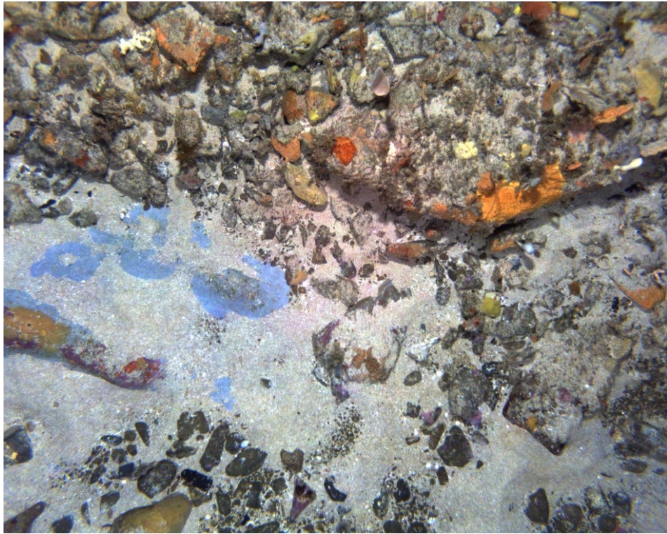
Figure 71. Low profile reef and mixed sand habitat with encrusting blue and orange sponges
