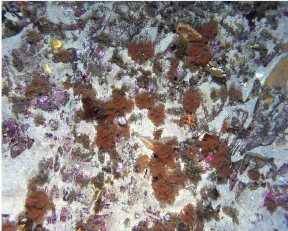
Figure 83. Sand inundated reef with soft bryozoa and red calcareous encrusting algae
