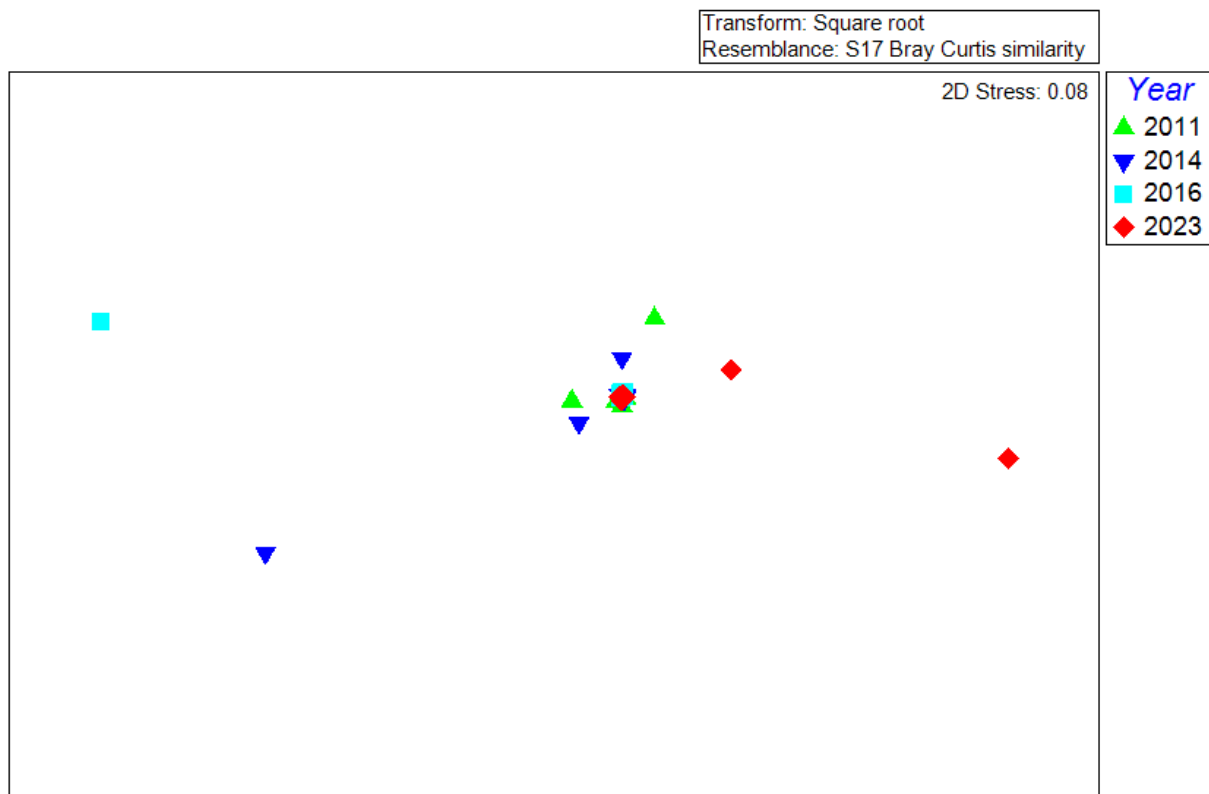
Figure 37. Non-metric multidimensional scaling plot showing community composition at Joe's Reef across survey years. Note that the majority of images are centred in the middle cluster (where symbols from all years are shown), with very few significant outliers between years.
