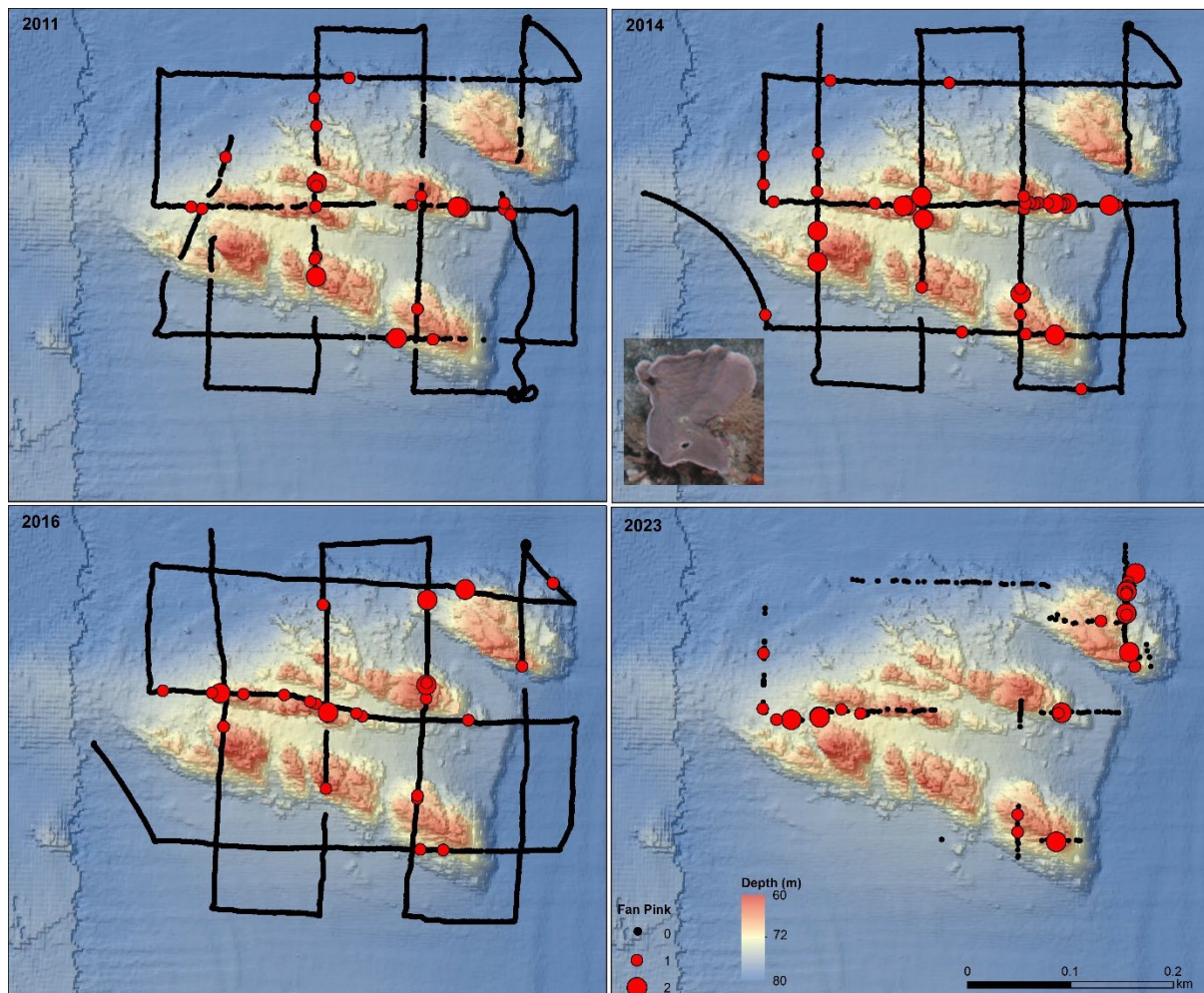
Figure 54. Changes in the spatial distribution in abundance (count per image) of fan pink sponges at Joe's Reef from targeted scoring. Note that the 2023 survey had incomplete coverage due to regular AUV failure in this complex terrain.
