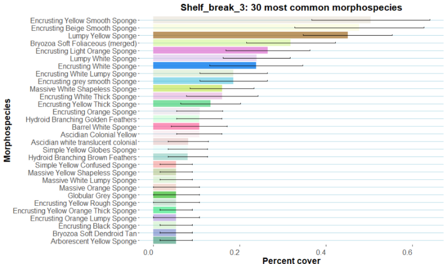
Figure 32. Percent cover (and standard error) of the thirty most common morphospecies at the Shelf break 3 transect. Biological matrix was excluded for improved visualisation.
