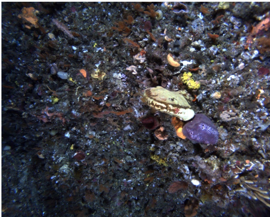
Figure 74. High profile reef with white fan thick sponge, massive purple sponge, and gorgonian red Pteronisis fans
