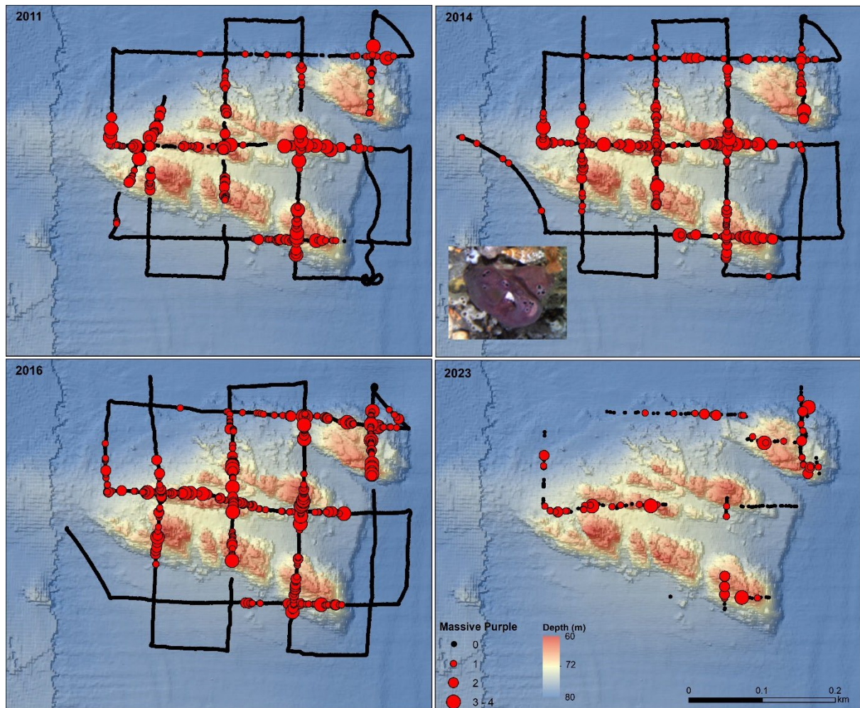
Figure 50. Changes in the spatial distribution in abundance (count per image) of massive purple sponges at Joe's Reef from targeted scoring. Note that the 2023 survey had incomplete coverage due to regular AUV failure in this complex terrain.
