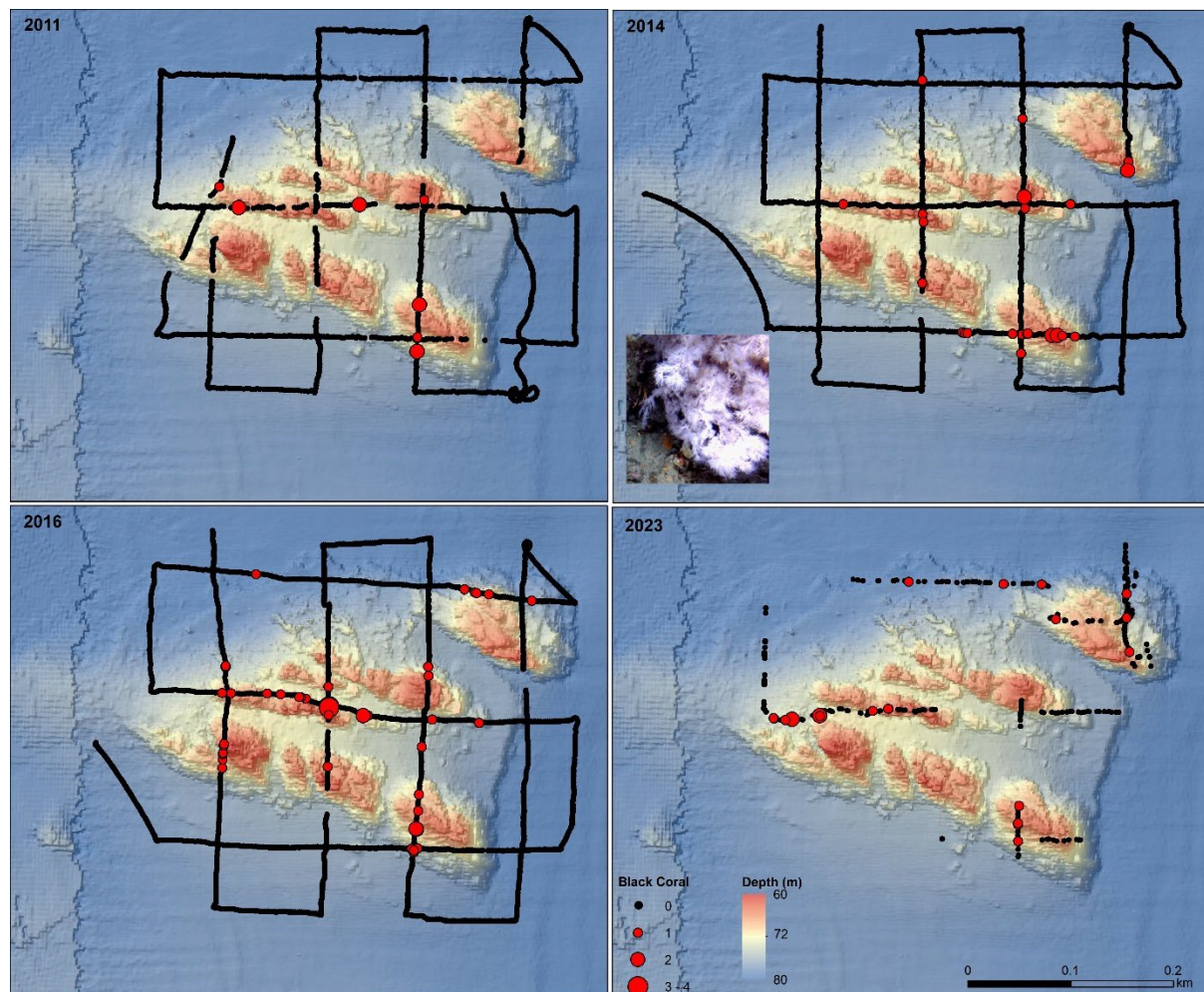
Figure 51. Changes in the spatial distribution in abundance (count per image) of black coral at Joe's Reef from targeted scoring. Note that the 2023 survey had incomplete coverage due to regular AUV failure in this complex terrain.
