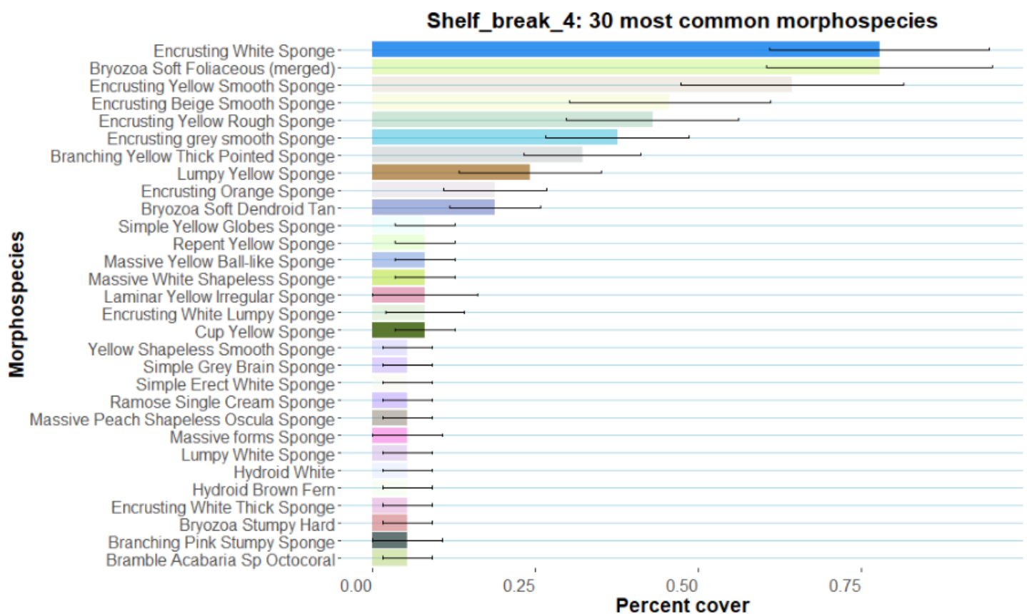
Figure 33. Percent cover (and standard error) of the 30 most common morphospecies at the Shelf break 4 transect. Biological matrix was excluded for improved visualisation.
