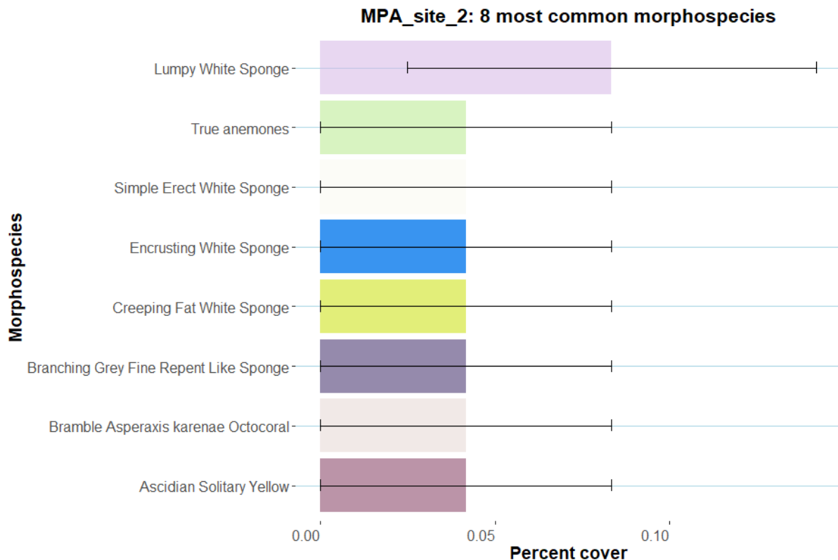
Figure 36. Percent cover (and standard error) of the eight most common morphospecies at the AMP site 2 transect. Biological matrix was excluded for improved visualisation.
