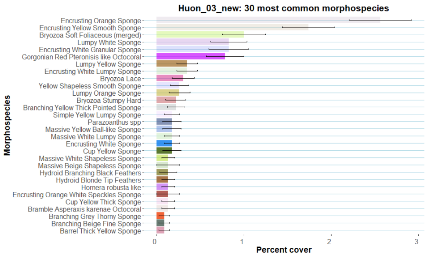
Figure 6. Percent cover (and standard error) of the 30 most common morphospecies annotated in the Huon_03_new transect in Huon Marine Park AUV imagery. The biological matrix category was excluded from the plot for improved visualisation.
