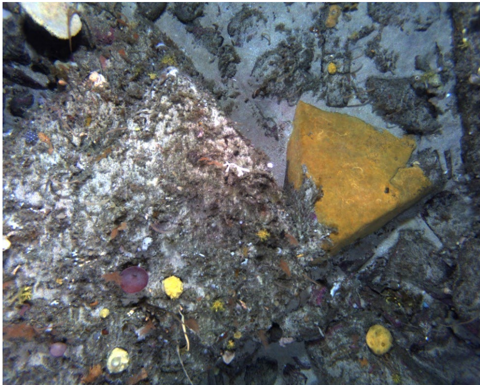
Figure 69. Moderate profile reef with encrusting yellow smooth sponge, biological matrix, red cup smooth sponge and other invertebrates
