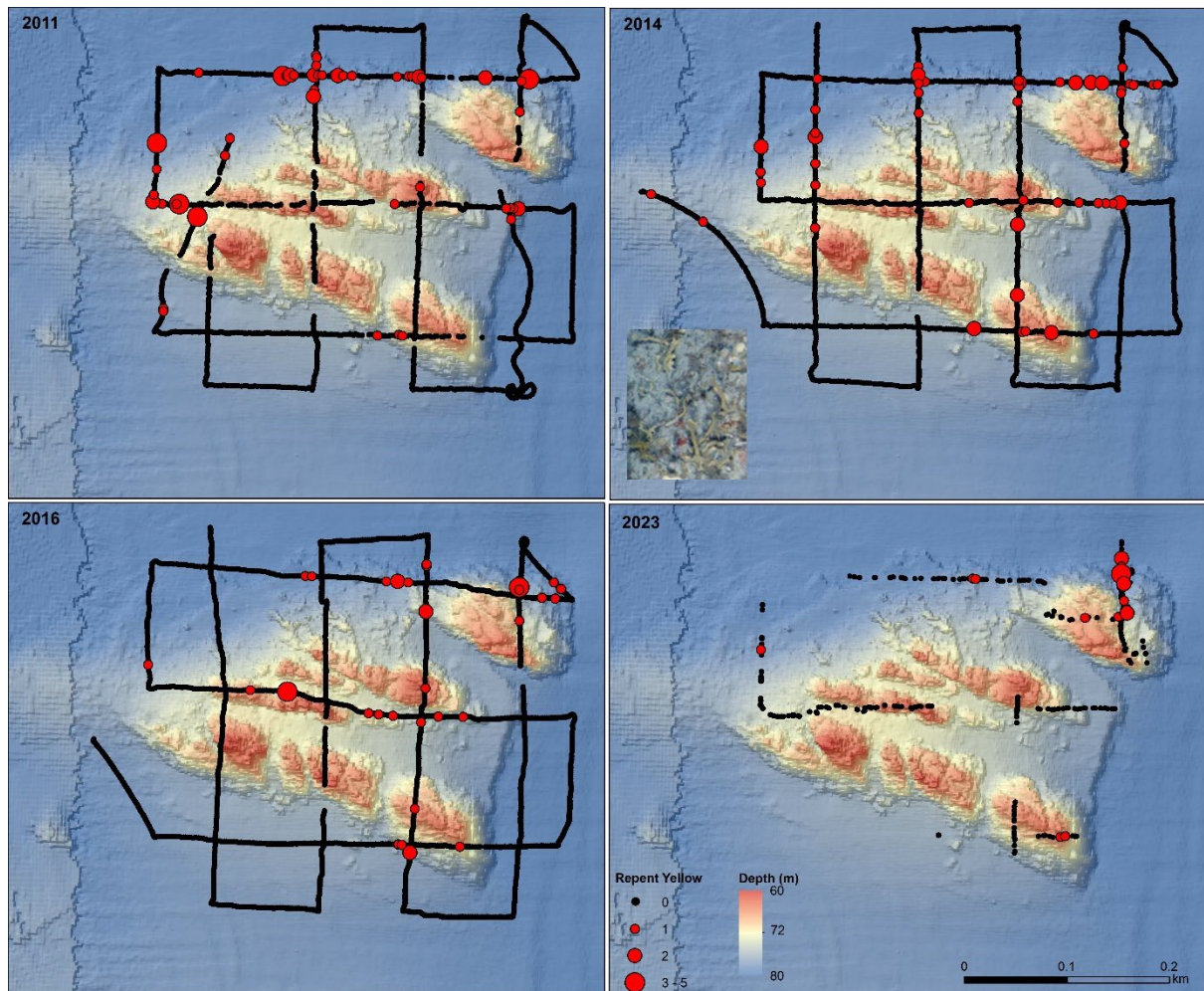
Figure 55. Changes in the spatial distribution in abundance (count per image) of repent yellow sponges at Joe's Reef from targeted scoring. Note that the 2023 survey had incomplete coverage due to regular AUV failure in this complex terrain.
