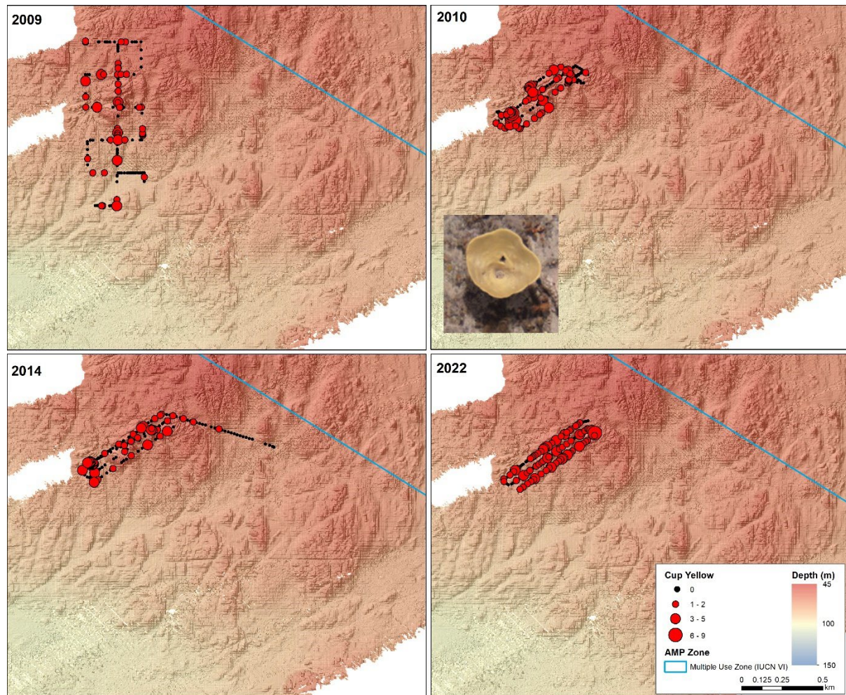
Figure 24. Changes in the spatial distribution in abundance (count per image) of cup yellow sponges at Huon_13 transect from targeted scoring. Note that a different transect design was used in the 2009 survey compared to subsequent surveys.
