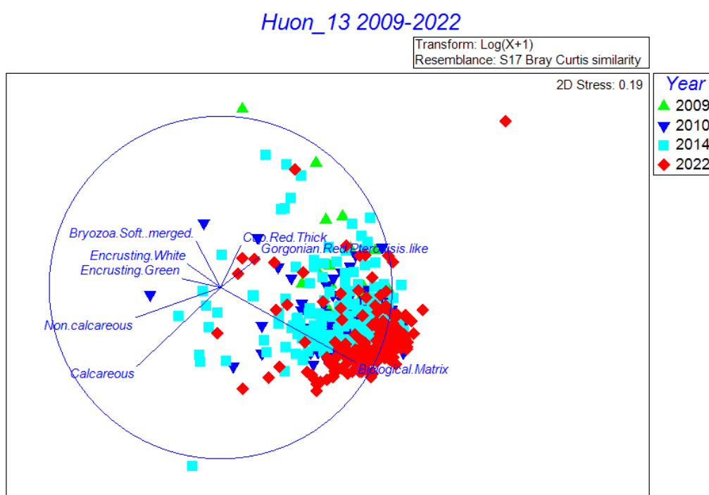
Figure 11. Non-metric multidimensional scaling plot showing community composition in Huon_13 transect across survey years.
