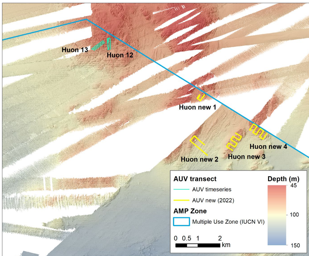
Figure 1. Locations of AUV transects in Huon Marine Park, including repeat time series and new extended coverage.
