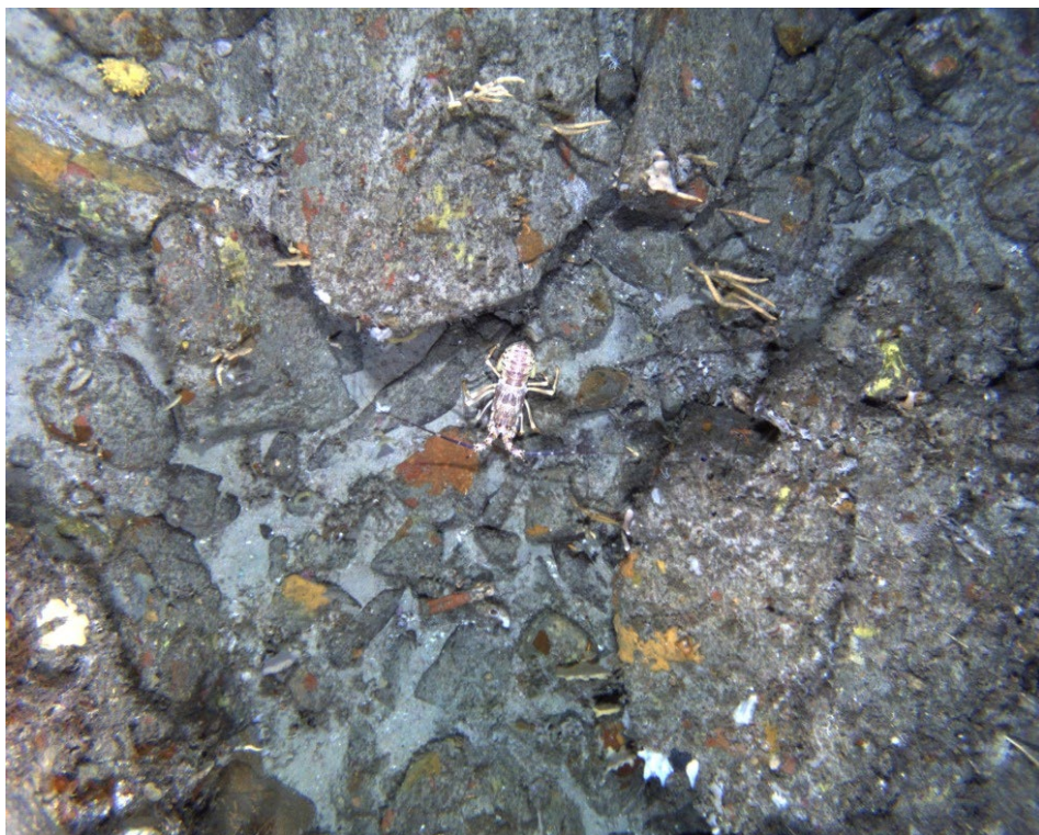
Figure 82. Moderate profile boulder reef habitat with rock lobster, branching and encrusting sponges and biological matrix
