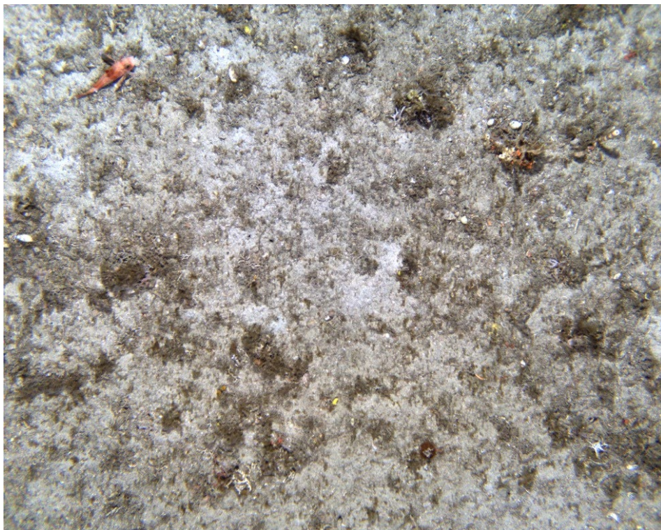
Figure 112. Sand and bryozoan rubble habitat with low cover of bryozoa/hydroid matrix and ocean perch
