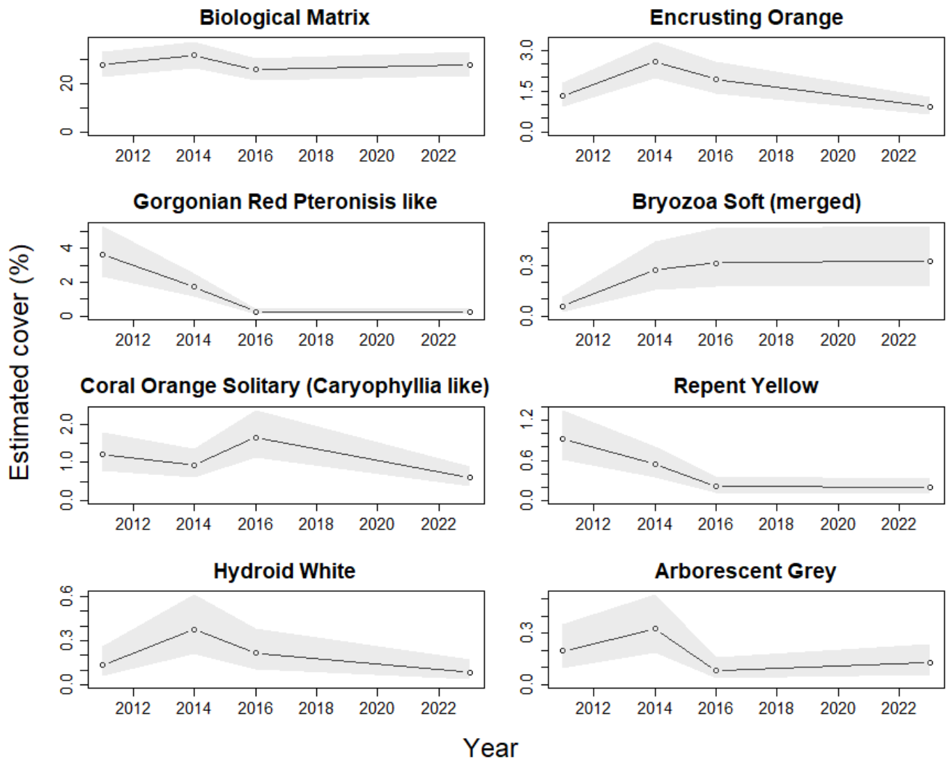
Figure 38. Model-based estimate of the temporal trend in the cover of the eight dominant morphospecies (including the grouping of biological matrix and soft bryozoa) at Joe's Reef. Points and lines show the mean and shaded area shows the 95% credible intervals. Estimates were made at the mean depth of the transect, ignoring any spatial effects. Note the differing scales on the y-axes.
