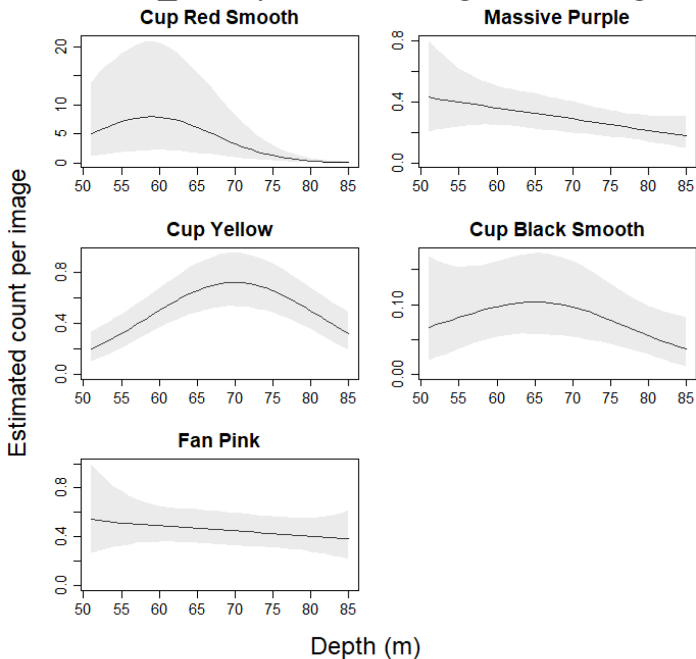
Figure 17. Relationship between the abundance of the five target scored morphospecies with depth at the Huon_13 site. Line shows the mean and shaded area shows the 95% credible intervals.
