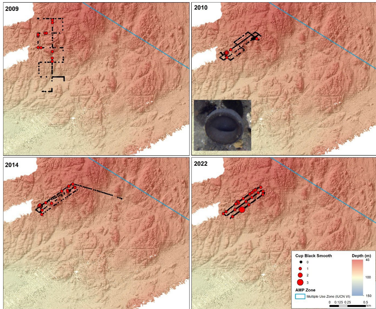
Figure 23. Changes in the spatial distribution in abundance (count per image) of cup black smooth sponges at Huon_13 transect from targeted scoring. Note that a different transect design was used in the 2009 survey compared to subsequent surveys.
