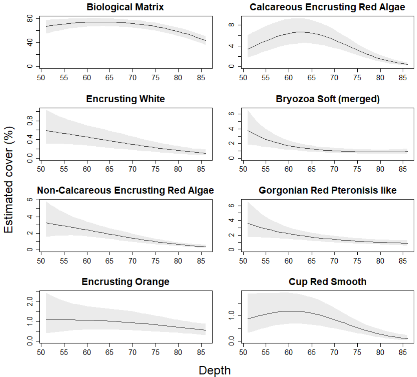
Figure 15. Relationship between the cover of the eight dominant morphospecies (including the grouping of biological matrix and soft bryozoa) with depth at the Huon_13 site. Line shows the mean and shaded area shows the 95% credible intervals. Note the differing scales on the y-axes.
