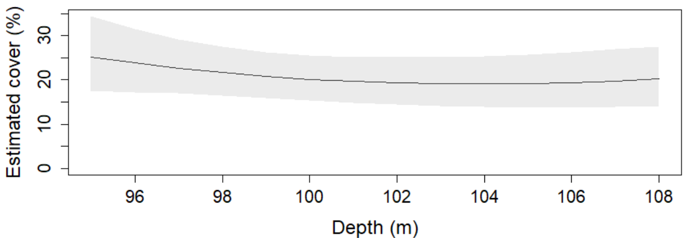
Figure 43. Relationship between the cover of biological matrix and depth at AMP site 2. Line shows the mean and shaded area shows the 95% credible intervals.
