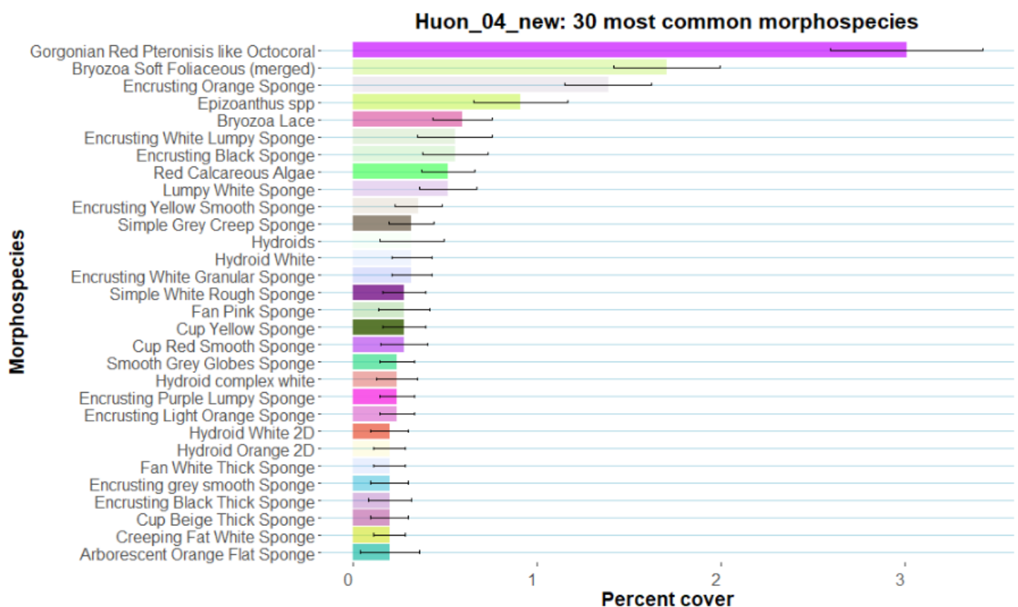
Figure 7. Percent cover (and standard error) of the 30 most common morphospecies annotated in the Huon_04_new transect in Huon Marine Park AUV imagery. The biological matrix category was excluded from the plot for improved visualisation.
