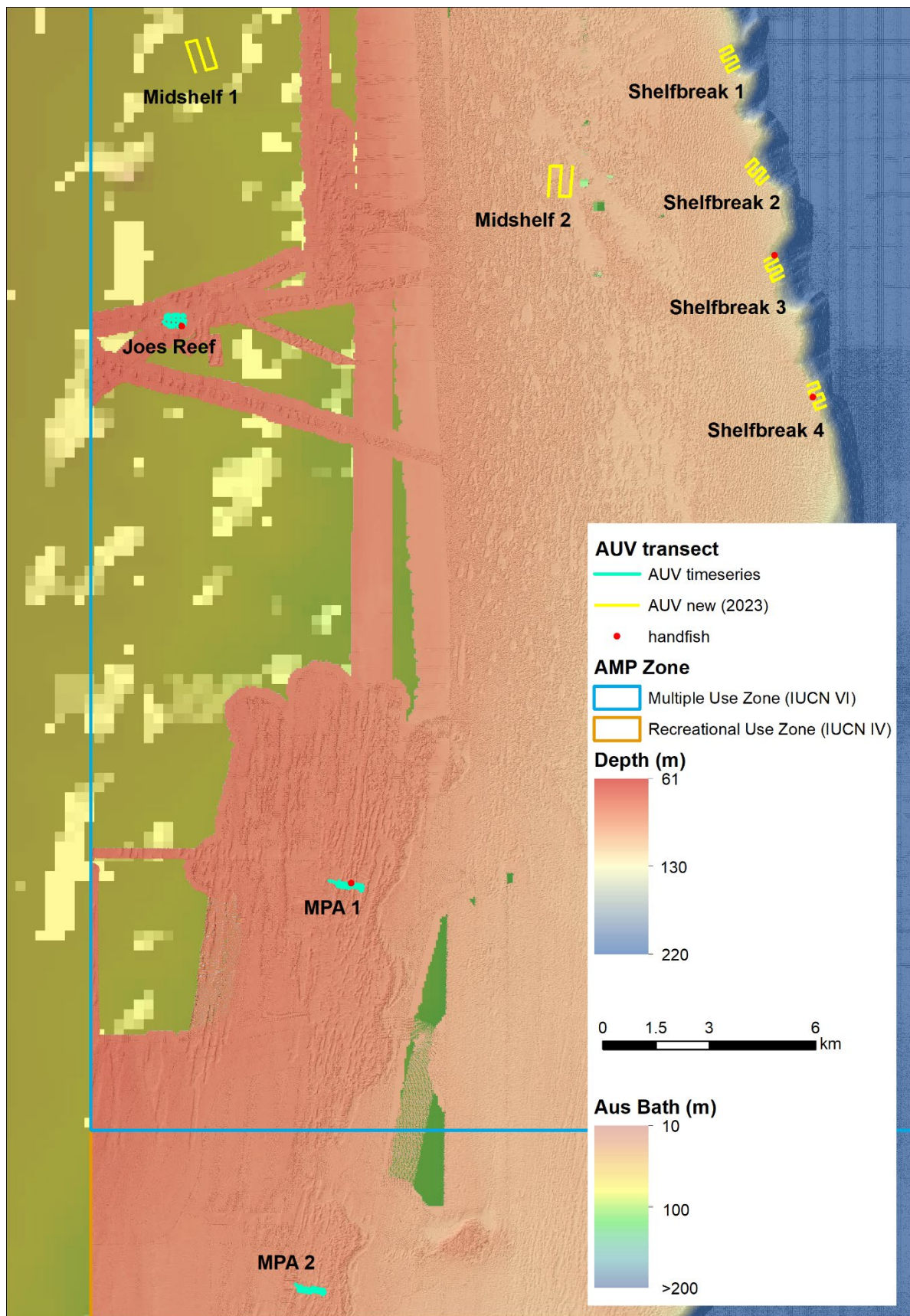
Figure 57. Location of handfish observed in FMP.
