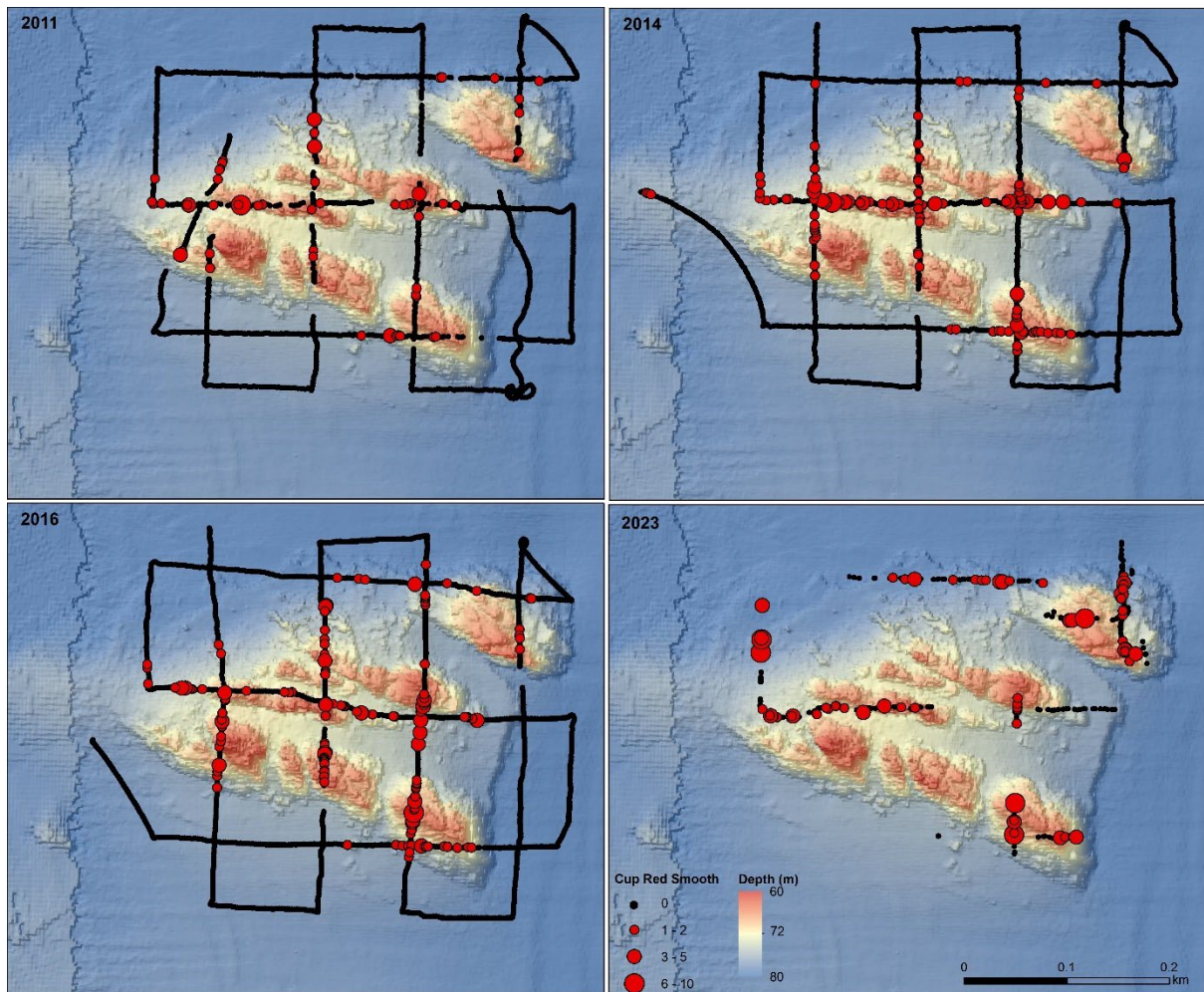
Figure 46. Changes in the spatial distribution in abundance (count per image) of cup red smooth sponges at Joe's Reef from targeted scoring. Note that the 2023 survey had incomplete coverage due to regular AUV failure in this complex terrain.
