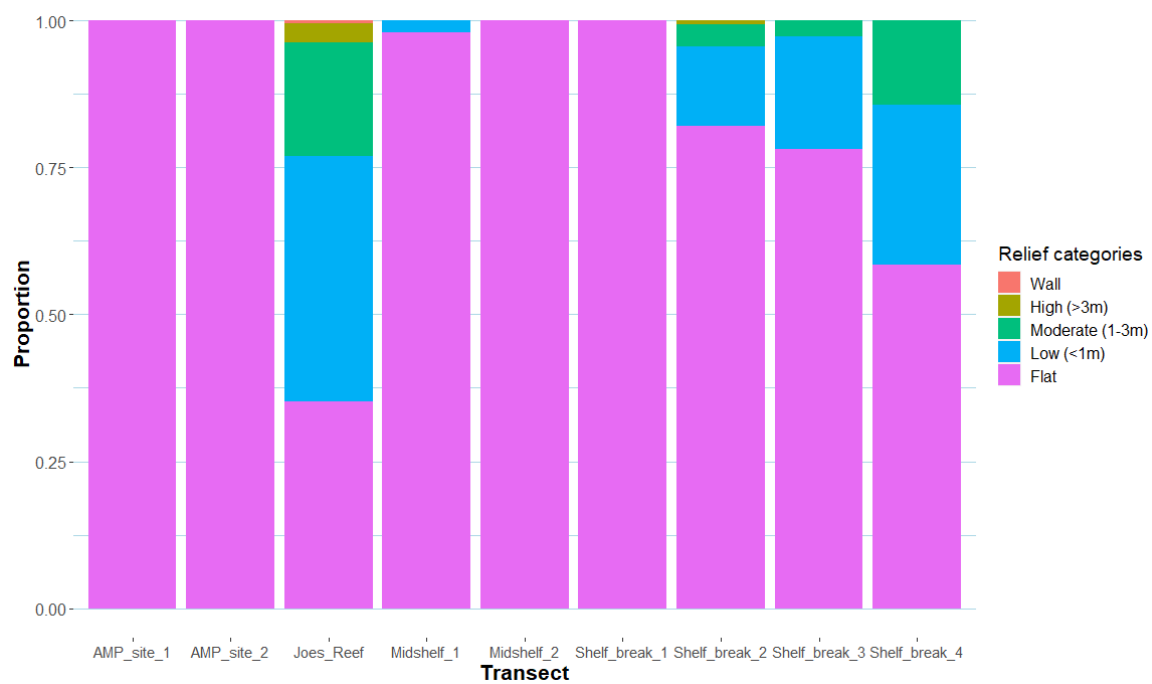
Figure 27. Summary of relief categories for images scored across each transect in Freycinet Marine Park.
