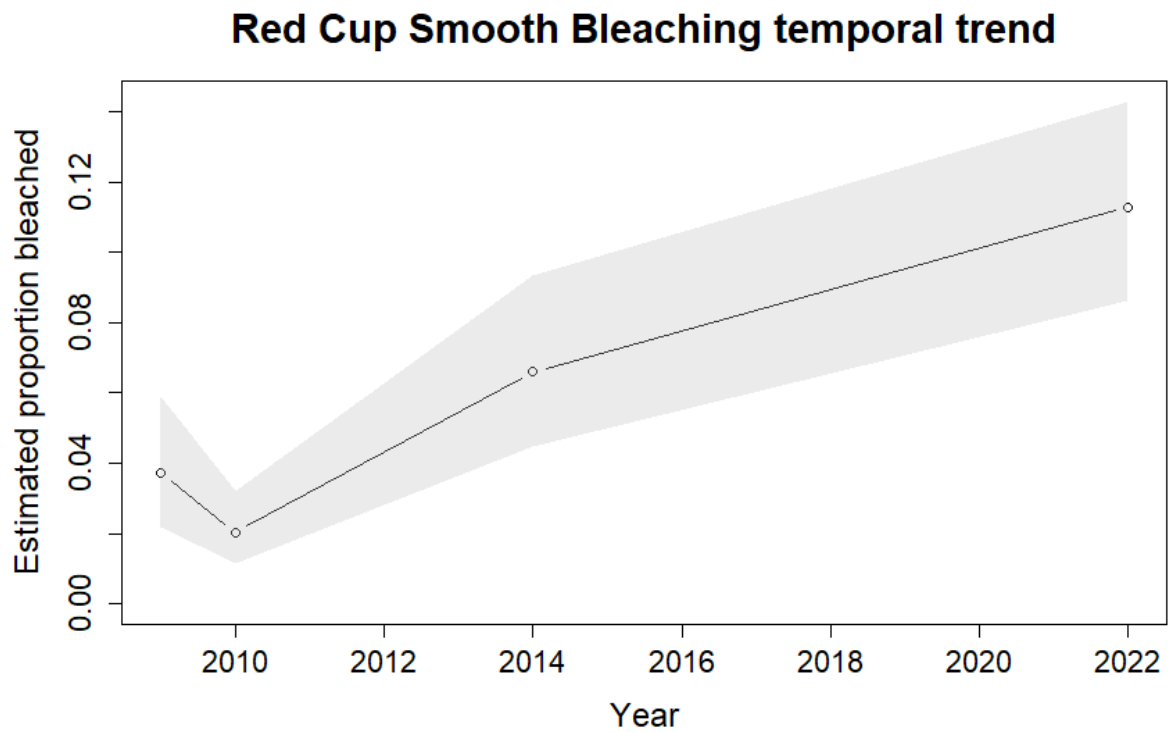
Figure 20. Temporal trend in the proportion of bleaching in cup red smooth sponges at the Huon_13 site from targeted scoring.
