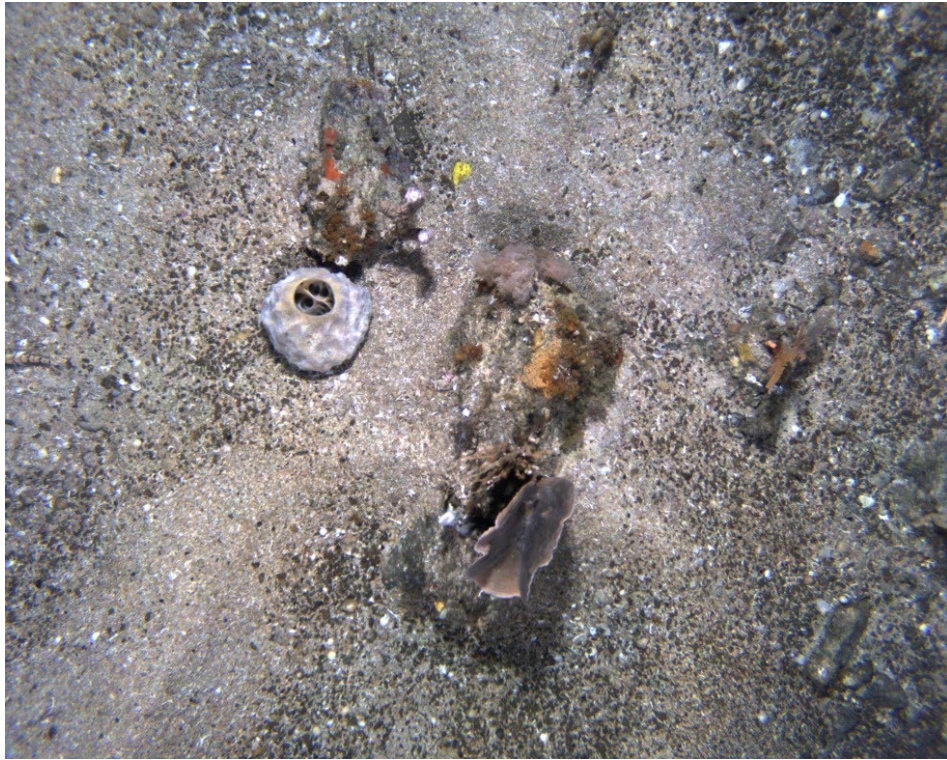
Figure 81. Mixed habitat of sand/pebble/reef with fan pink sponge and large white sponge
