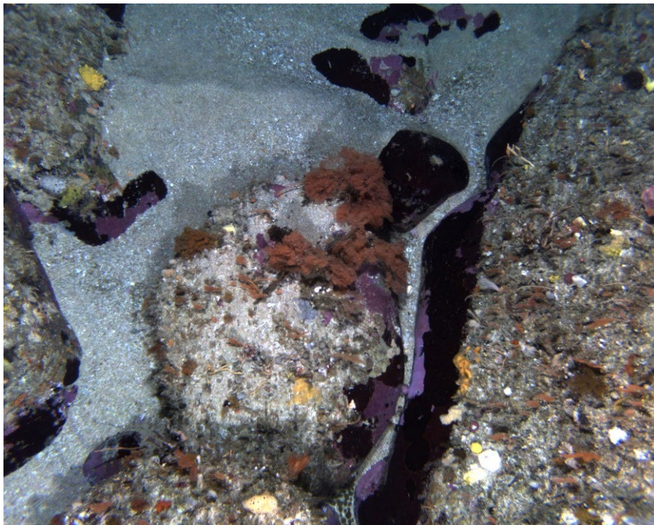
Figure 64. Southern rock lobster on encrusting orange sponge and fan white sponge on low profile reef
